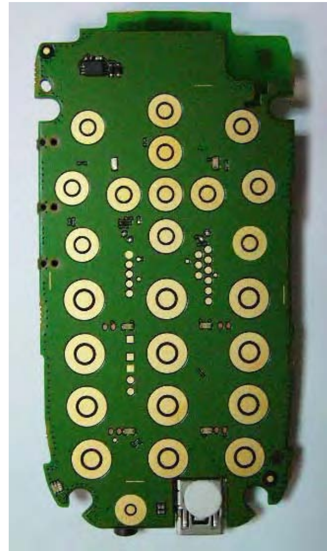
Front View
