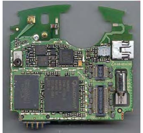
Front View (Shields Removed)
