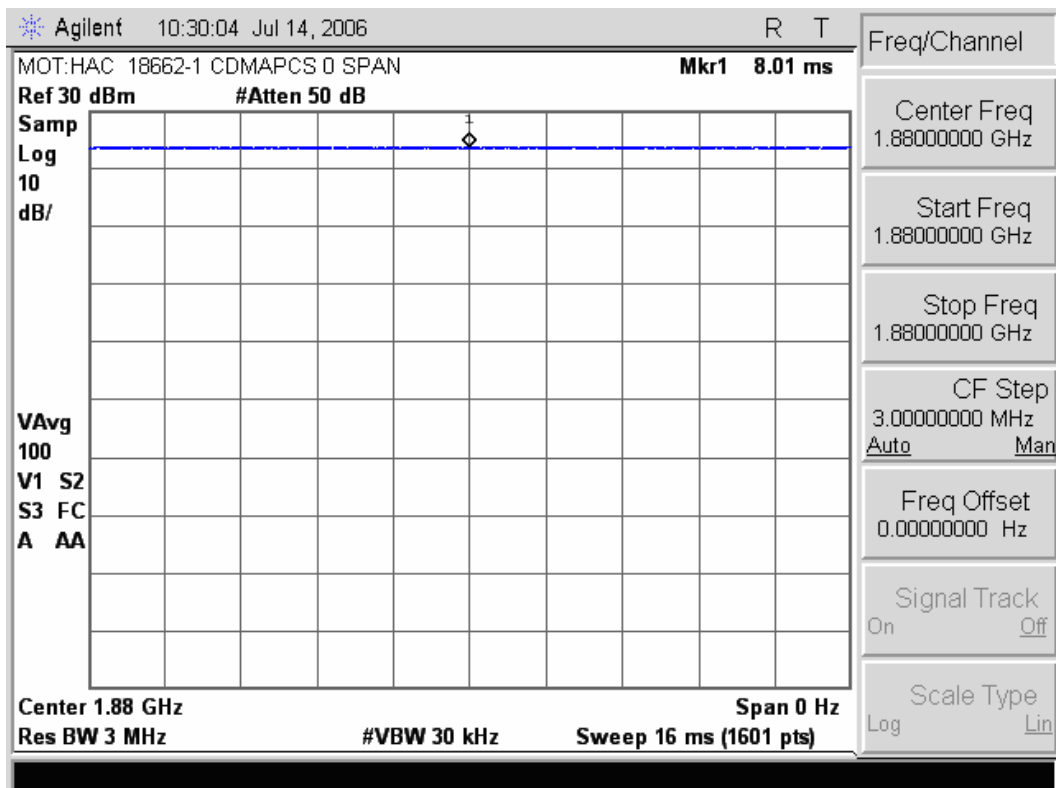
CDMA 1900 CH 600 (1880) 0 SPAN
