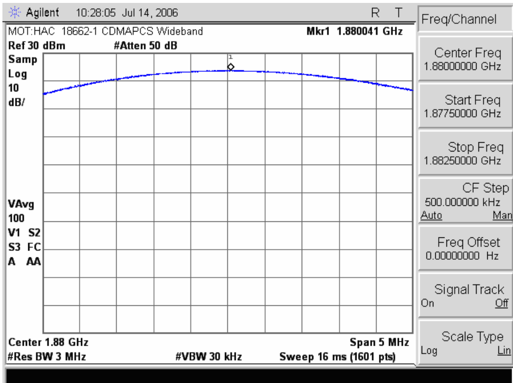
CDMA 1900 CH 600 (1880) WIDEBAND
