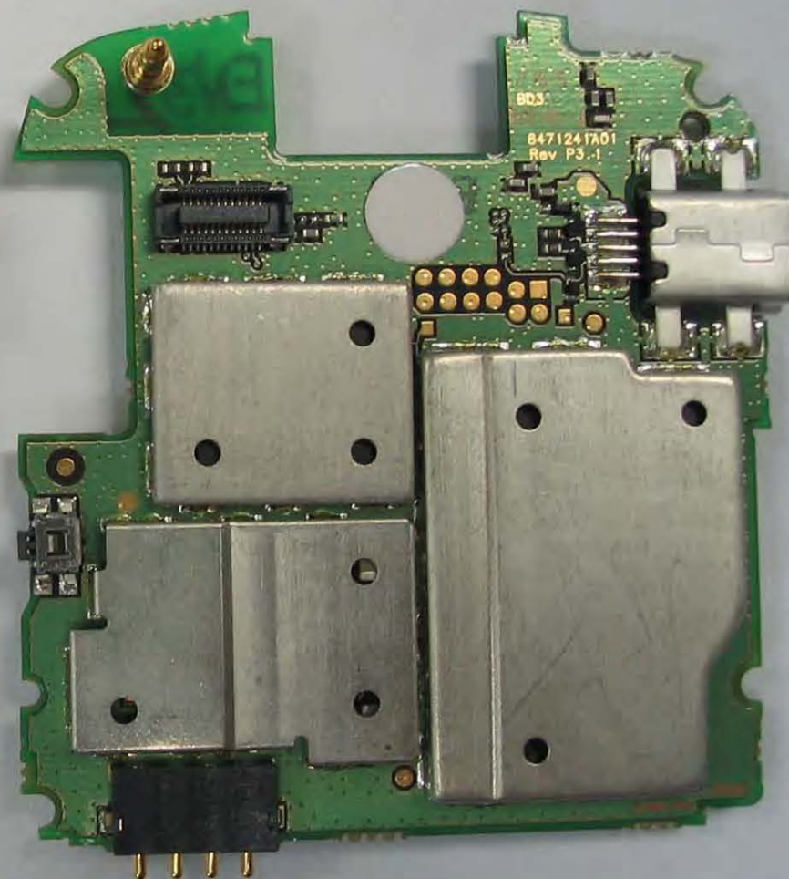
Main PCBA (Rear View)
