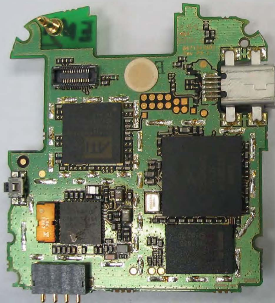
Rear View With Shields Removed
