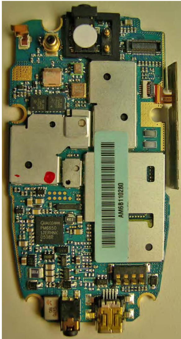
Main Board Bottom
