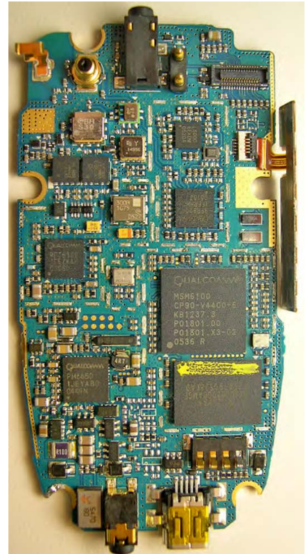
Main Board Bottom without Shields
