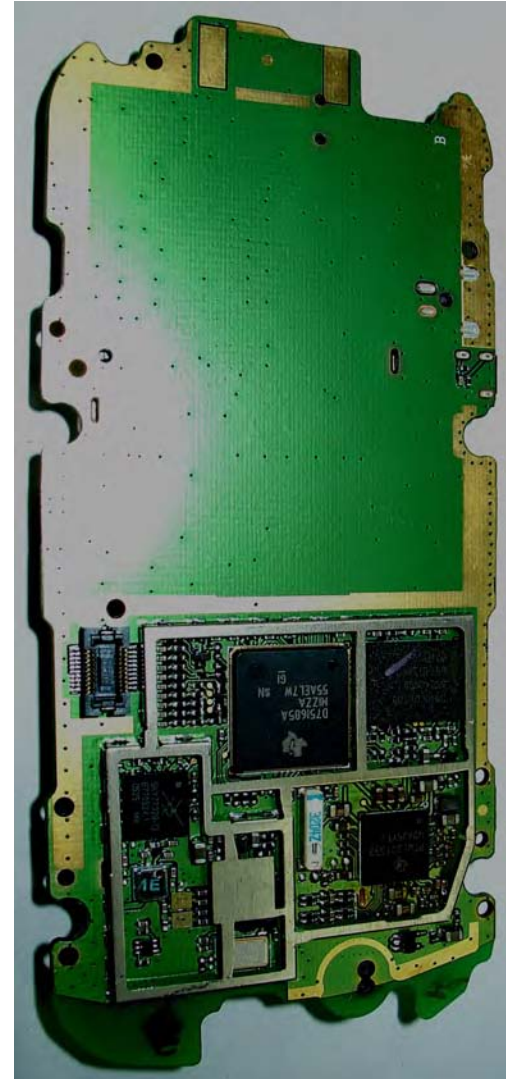
Main Board Top
