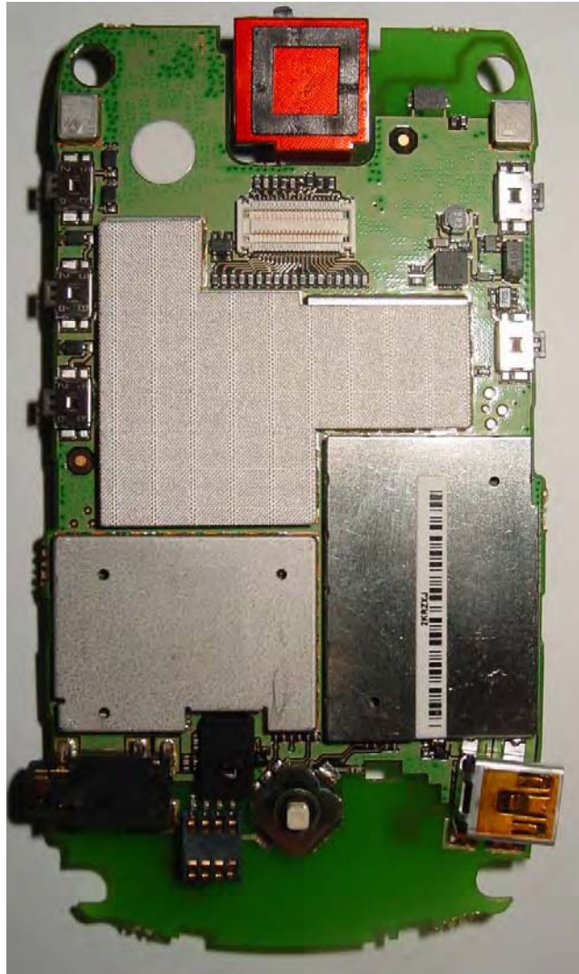
Main Board Top
