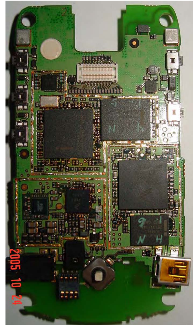
Main Board Top without Shields
