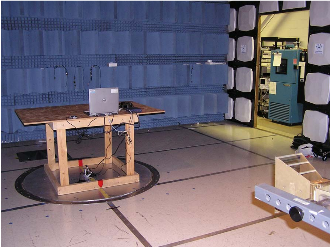
Radiated Emissions Measurement Setup
