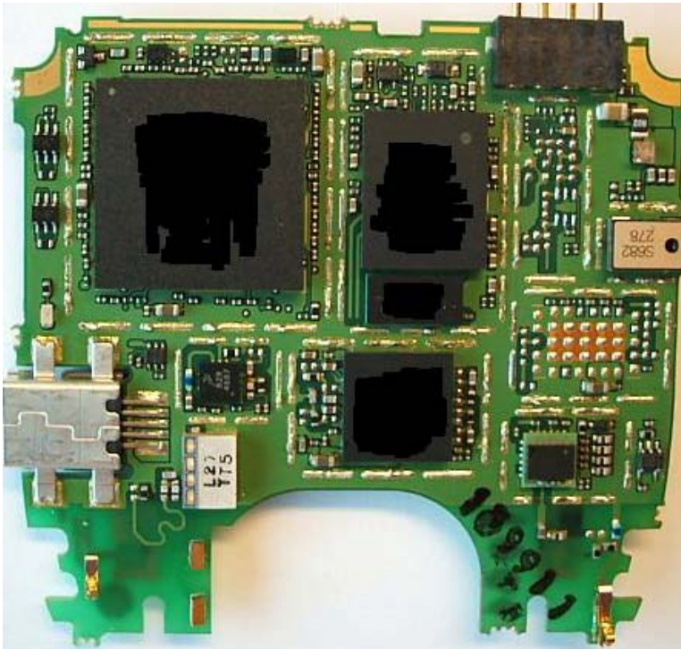
Main Board, Side B, Without Shields
