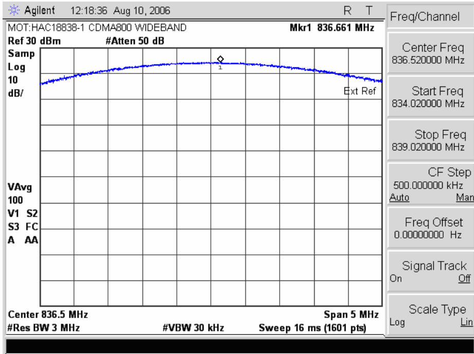
836.52 MHz (wideband)
