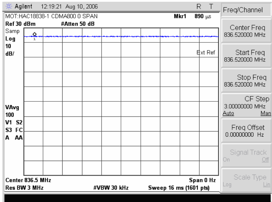
836.52 MHz (0 span)
