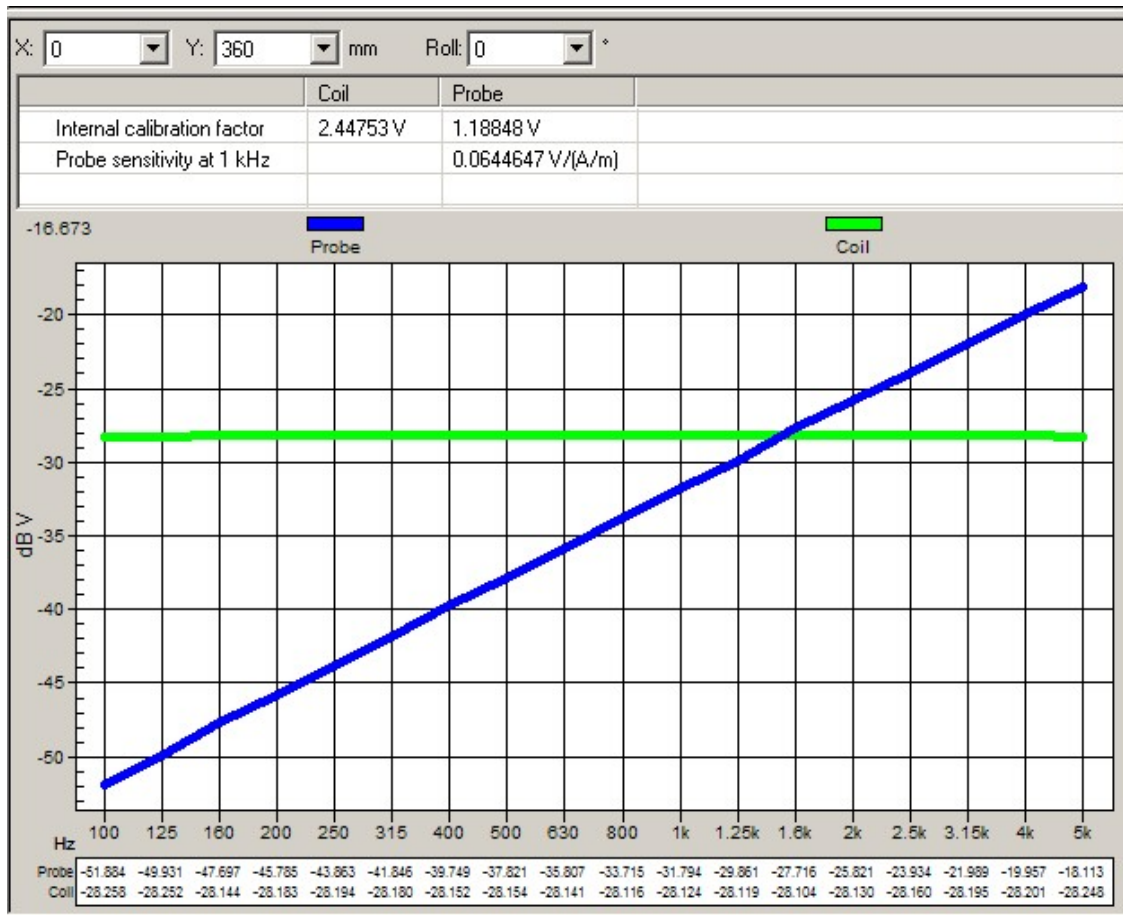
Graph 1: Frequency Response measured in AMCC
