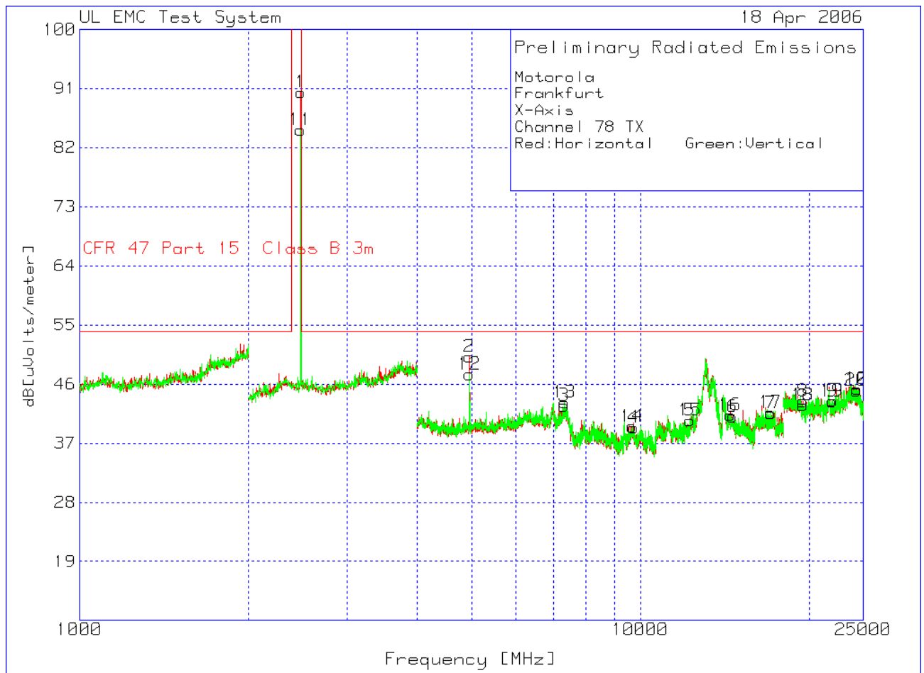
1-25 GHz High Channel Dual Polarization X
