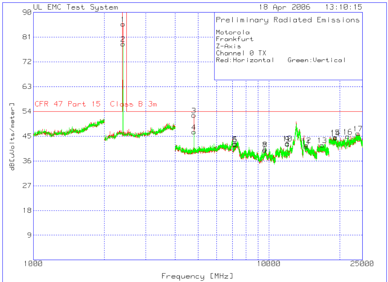
1-25 GHz Low Channel Dual Polarization Z
