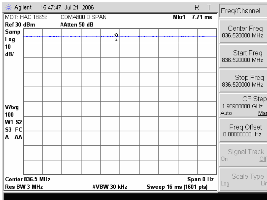
836.52 MHz (0 span)
