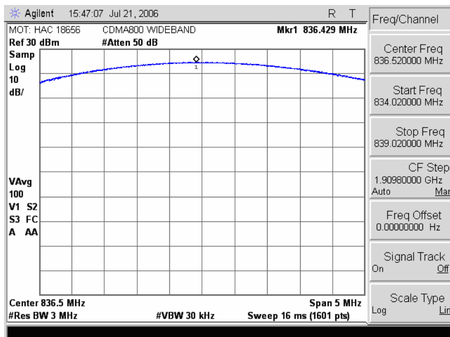
836.52 MHz (wideband)
