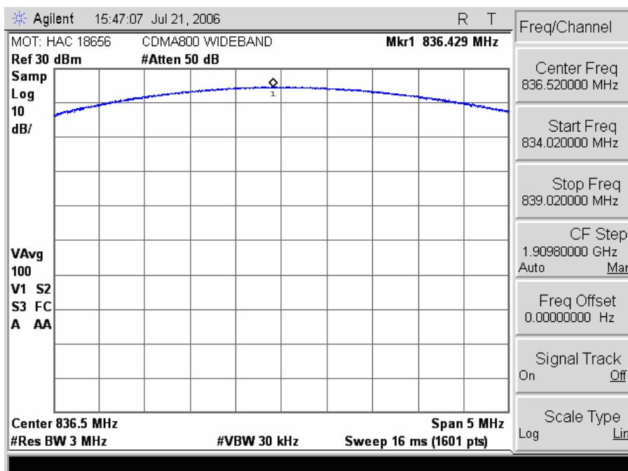
836.52 MHz (wideband)
