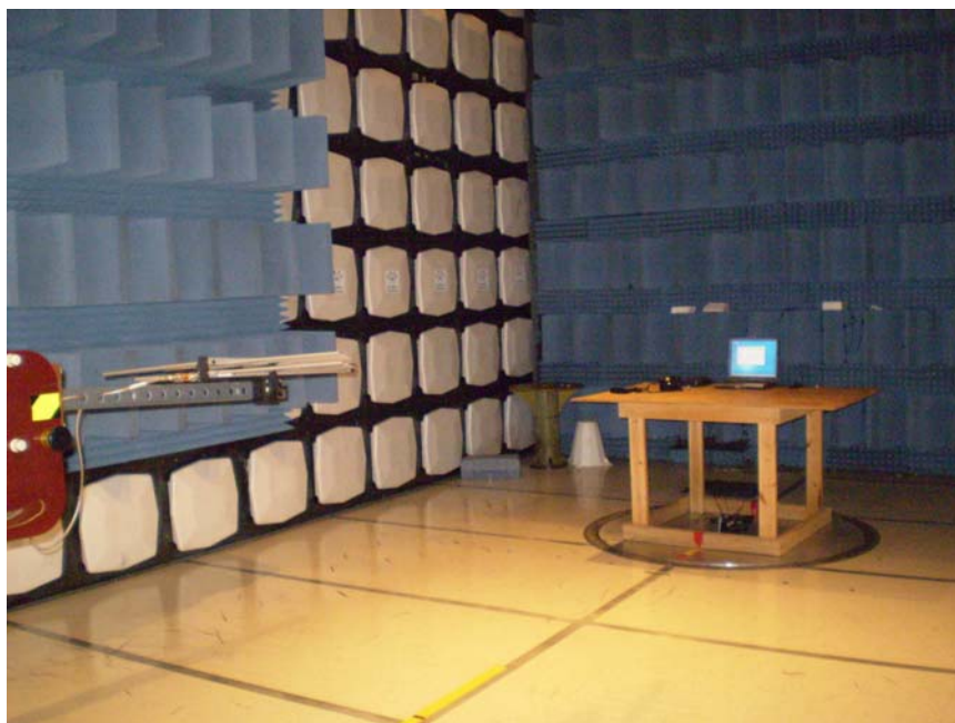
Figure 3. Computer Peripheral Part 15 Radiated Emissions Measurement Setup
