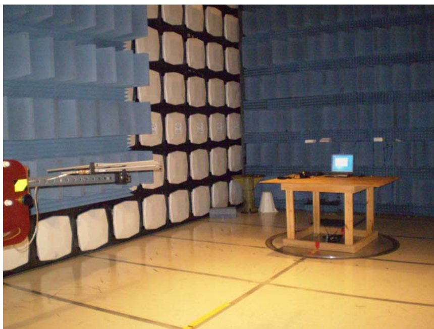
Figure 4. Part 22/24 Radiated Emissions Measurement Setup
