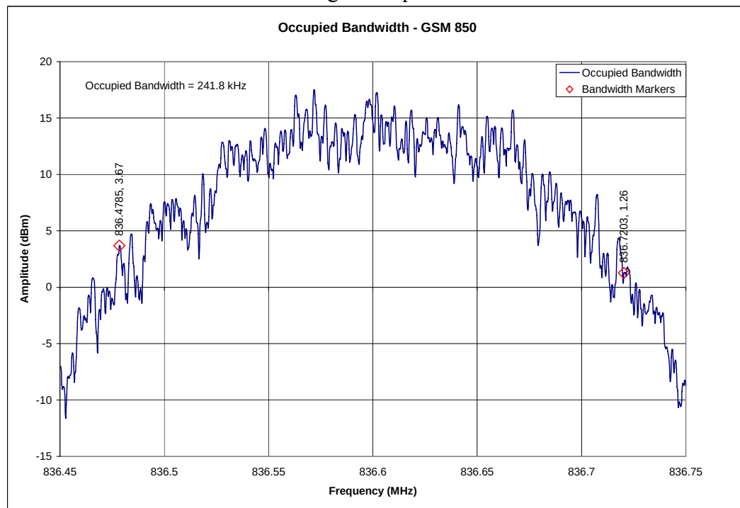
GSM 850 Edge Occupied Bandwidth
