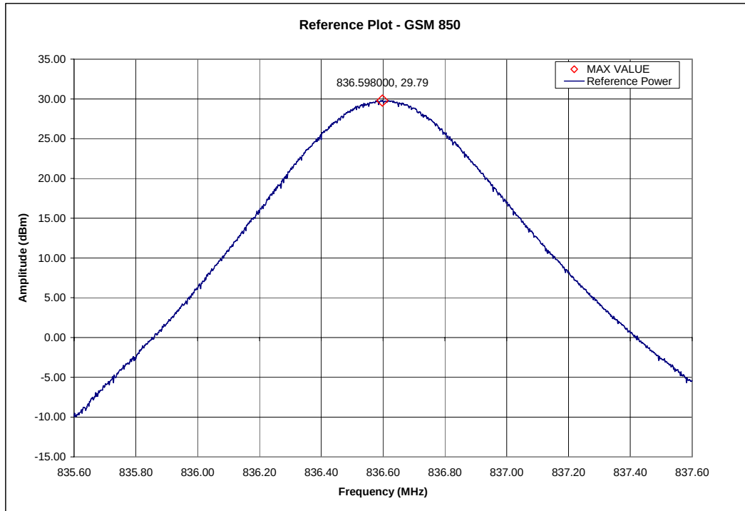
GSM 850 Edge Reference Plot
