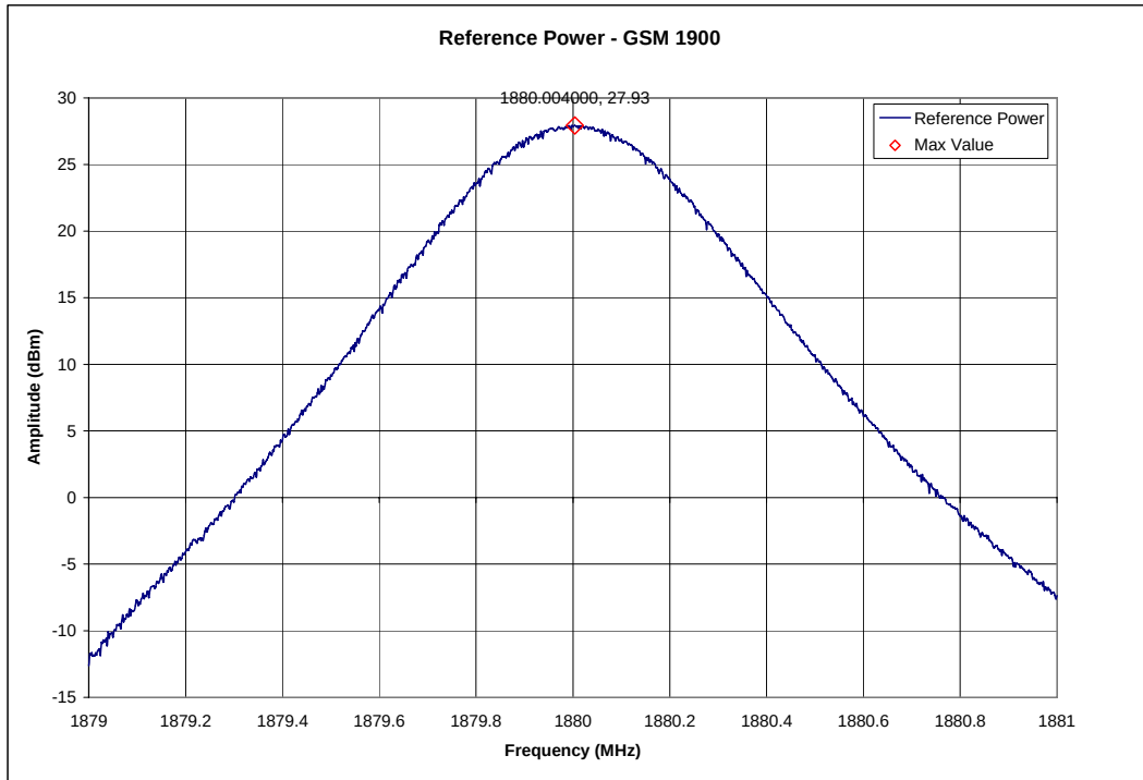
GSM 1900 Edge Reference Plot
