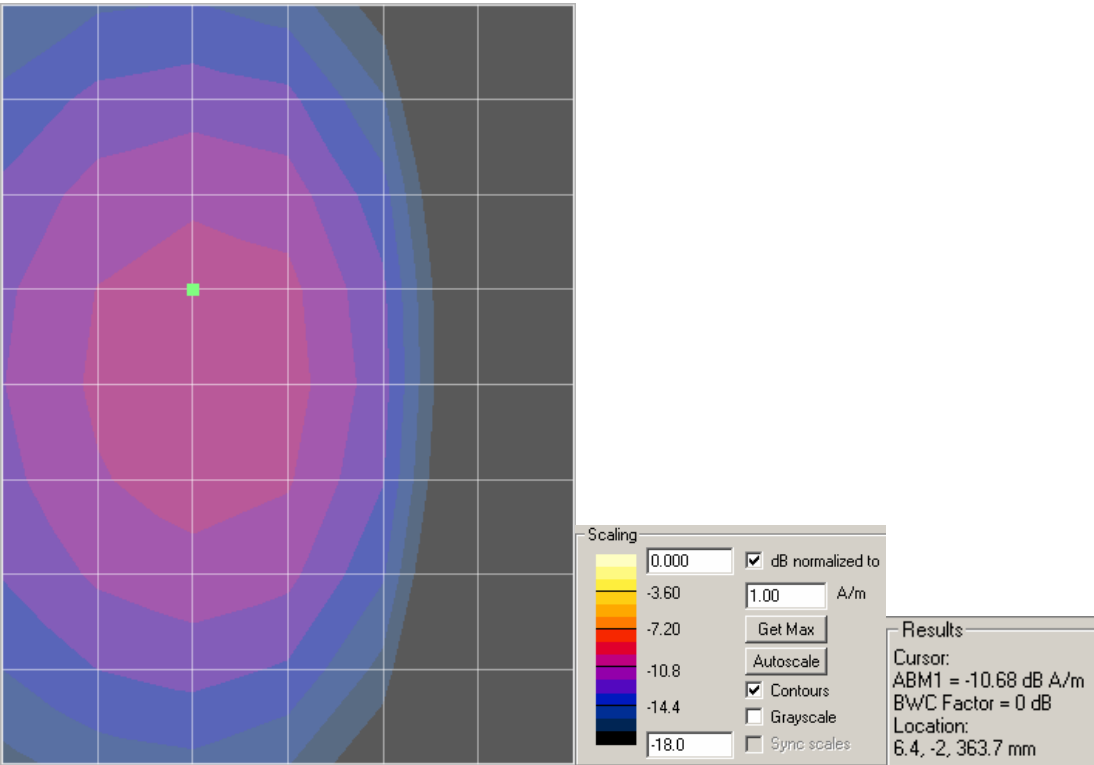
Radial 1 – ABM1
