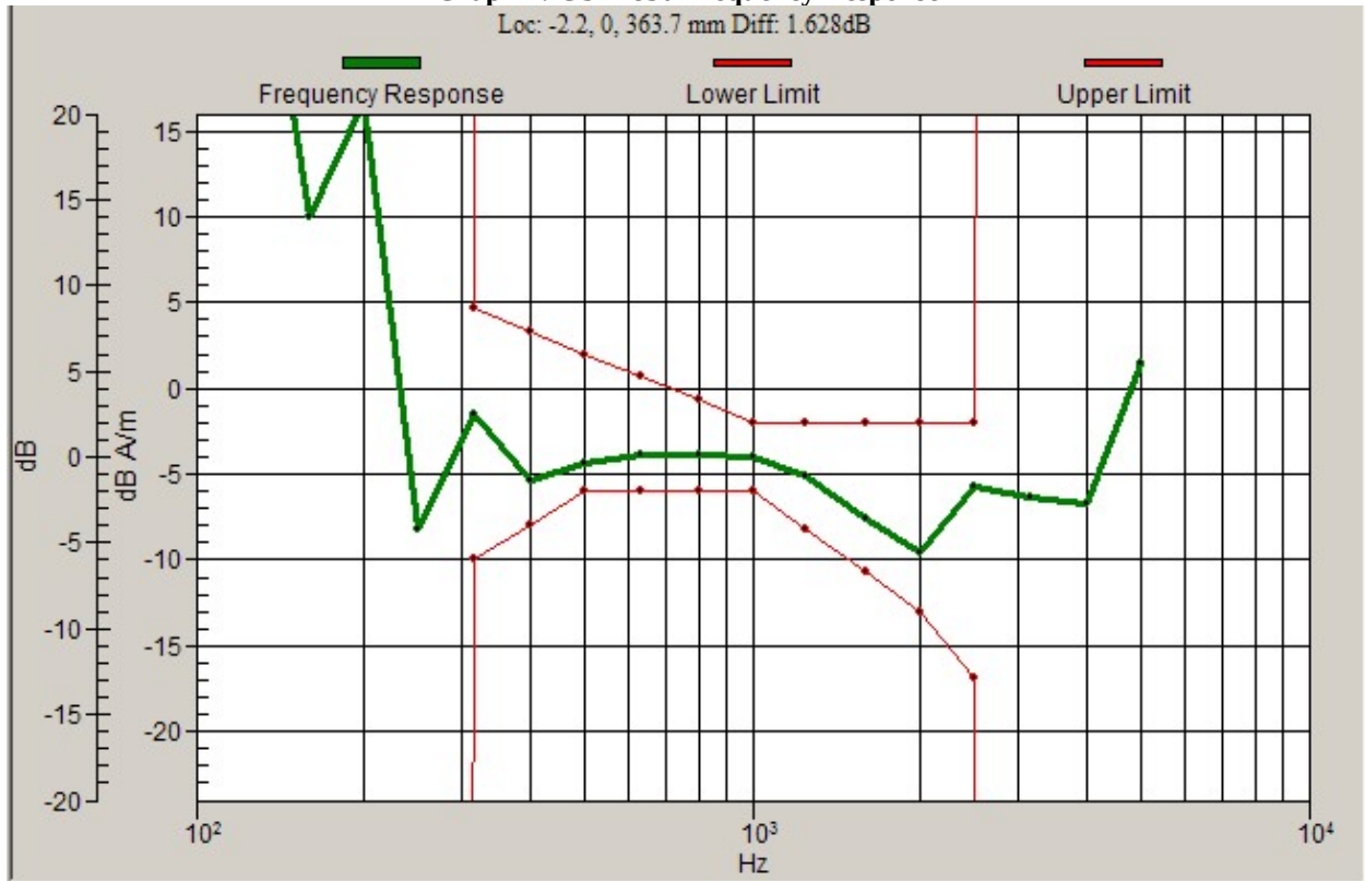
Graph 2: GSM 850 Frequency Response
