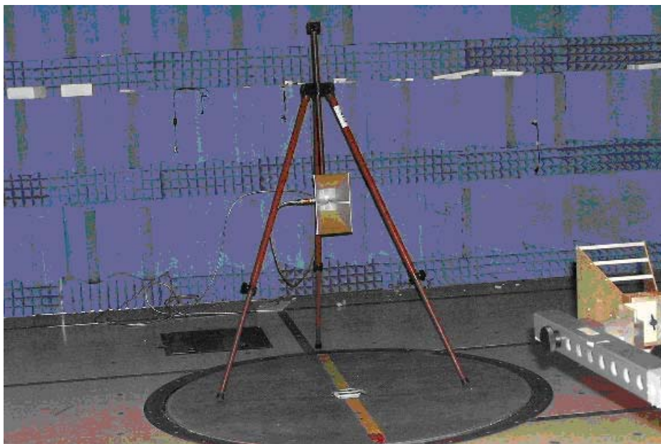
Figure 4. Antenna Substitution Method
