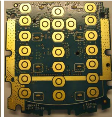
Key Board Bottom Without popples
