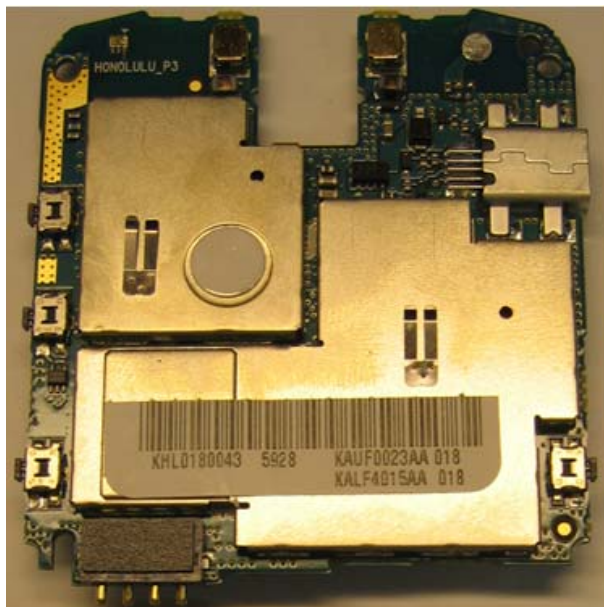
Main Board Bottom With Shields
