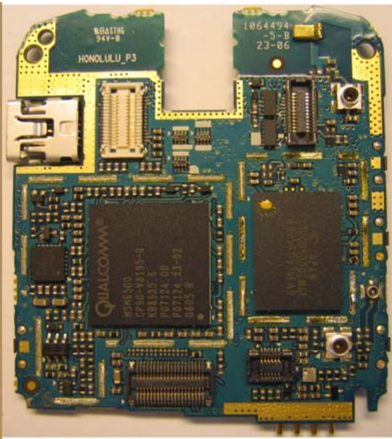
Main Board Top Without Shields
