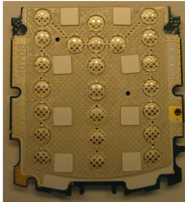
Key Board Bottom With popples
