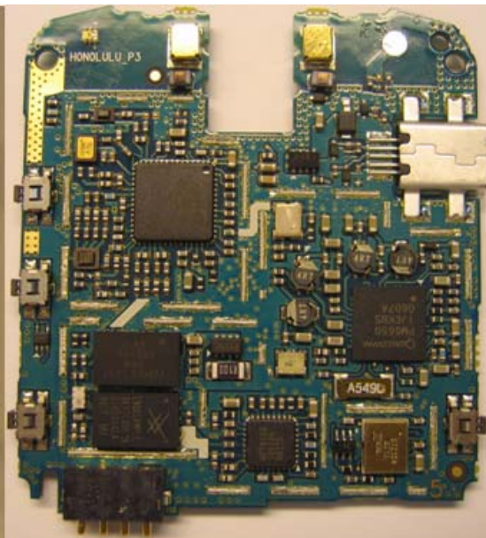
Main Board Bottom Without Shields
