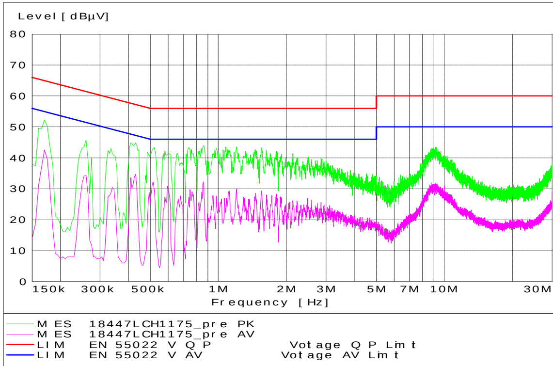
CDMA PCS Channel 1175 - Tx Mode - Line Coupling
