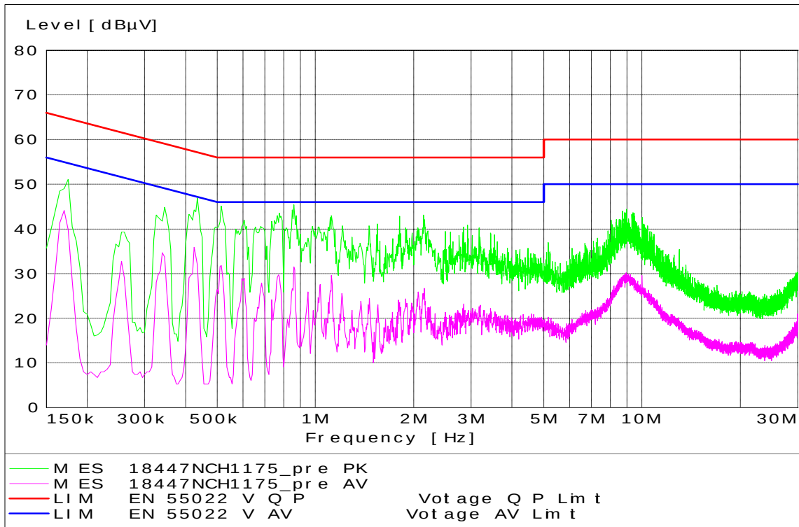
CDMA PCS Channel 1175 - Tx Mode - Neutral Coupling
