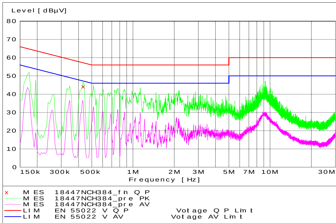
800 CDMA Channel 384 - Tx Mode - Neutral Coupling
