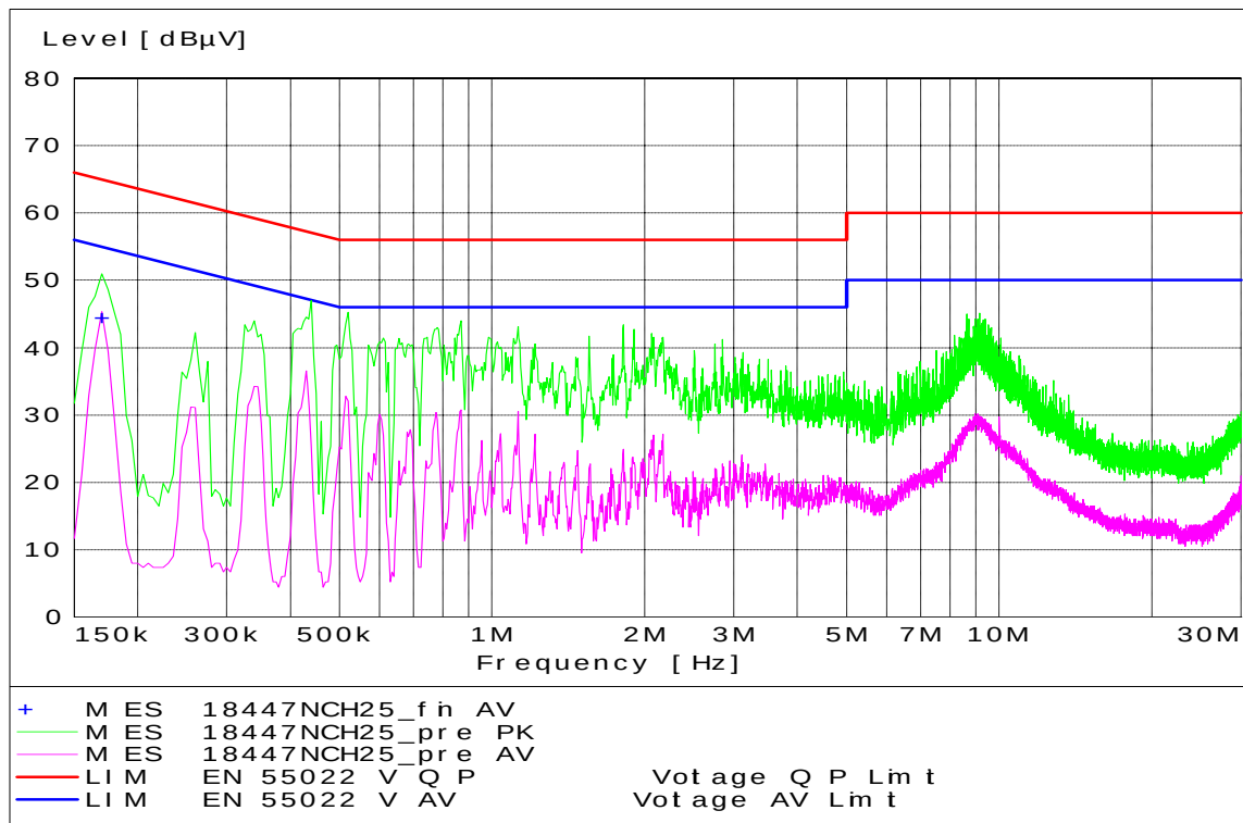
CDMA PCS Channel 25 - Tx Mode - Neutral Coupling
