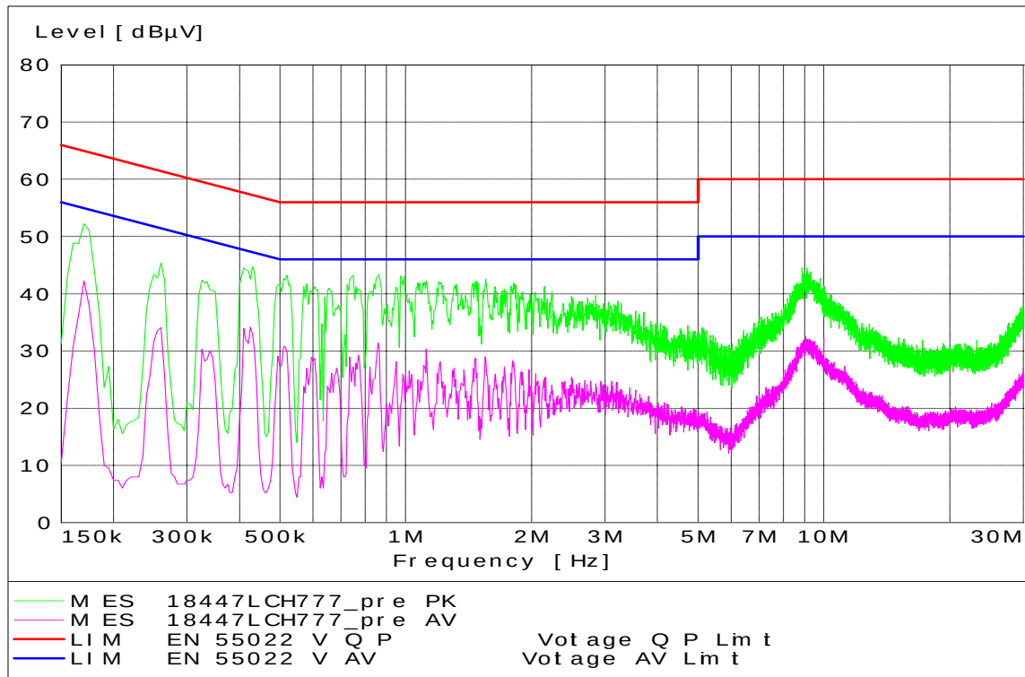
800 CDMA Channel 777 - Tx Mode - Line Coupling
