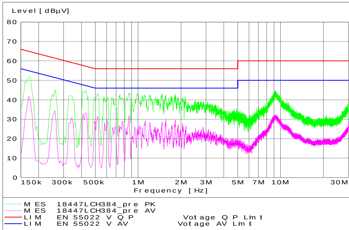
800 CDMA Channel 384 - Tx Mode - Line Coupling
