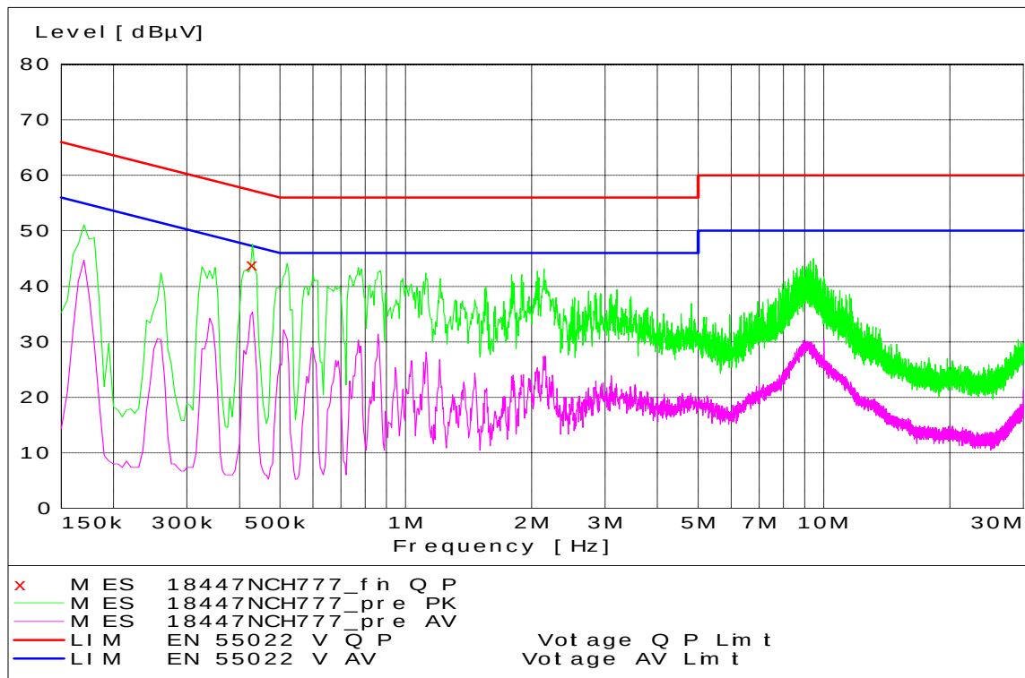
800 CDMA Channel 777 - Tx Mode - Neutral Coupling
