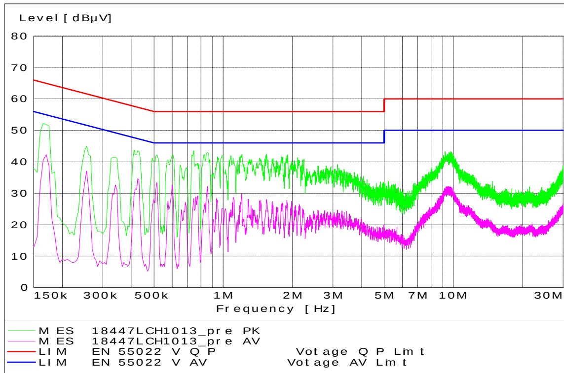
800 CDMA Channel 1013 - Tx Mode - Line Coupling
