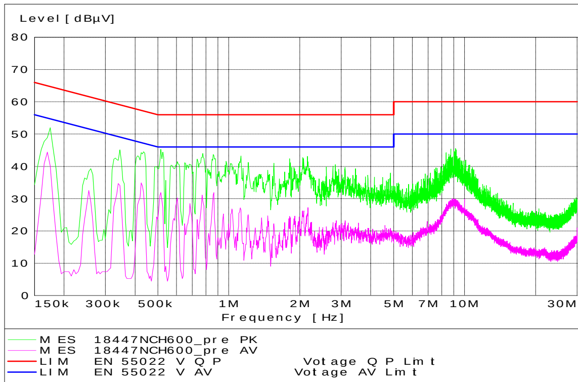
CDMA PCS Channel 600 - Tx Mode - Neutral Coupling
