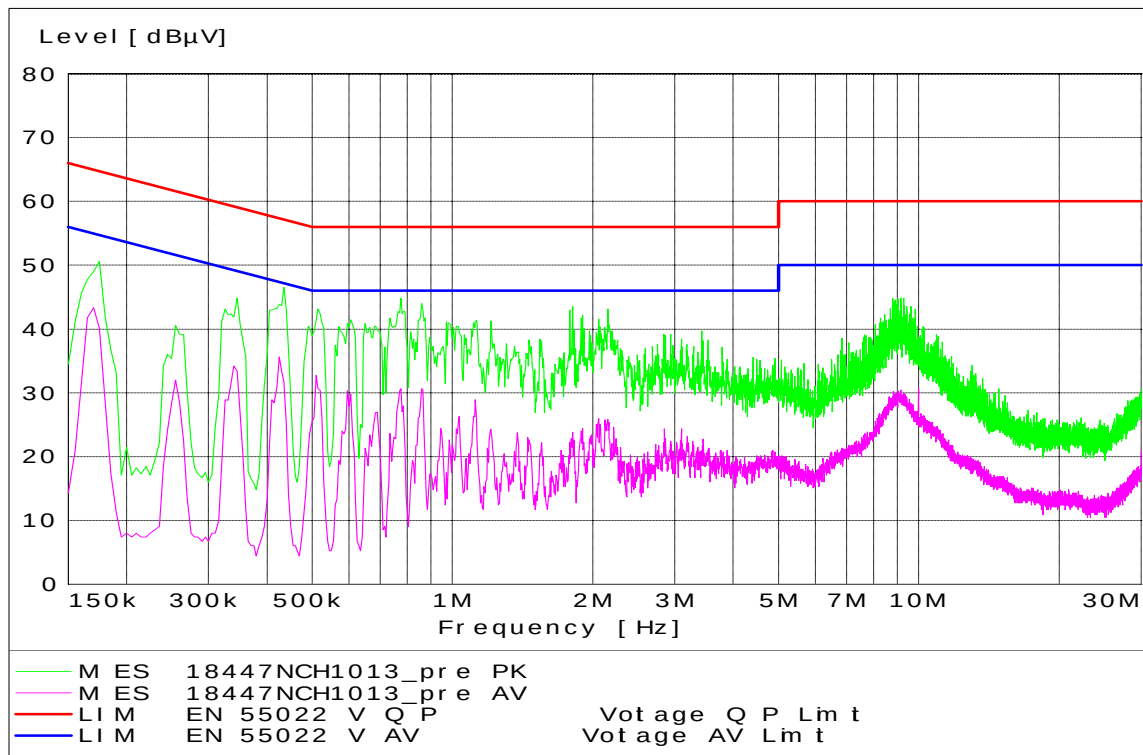
800 CDMA Channel 1013 - Tx Mode - Neutral Coupling
