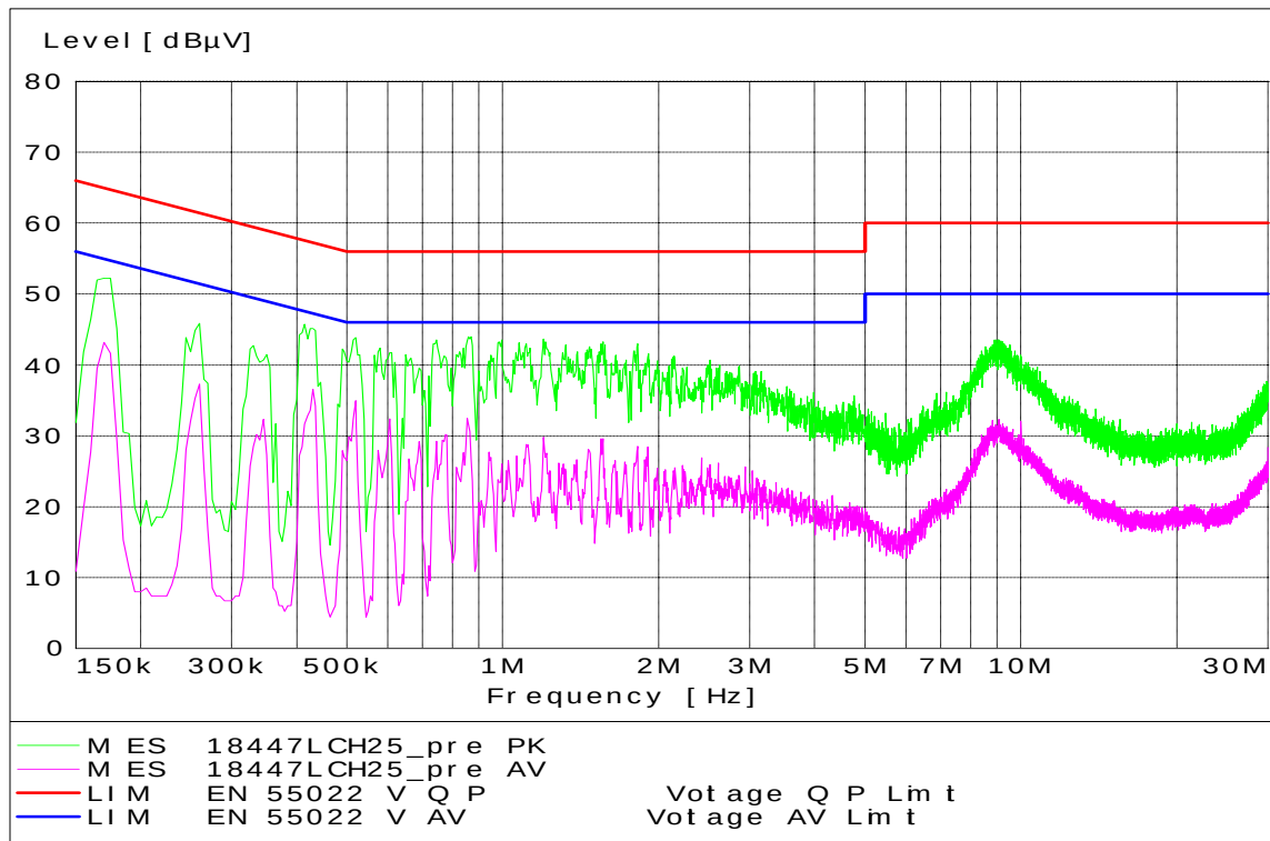
CDMA PCS Channel 25 - Tx Mode - Line Coupling
