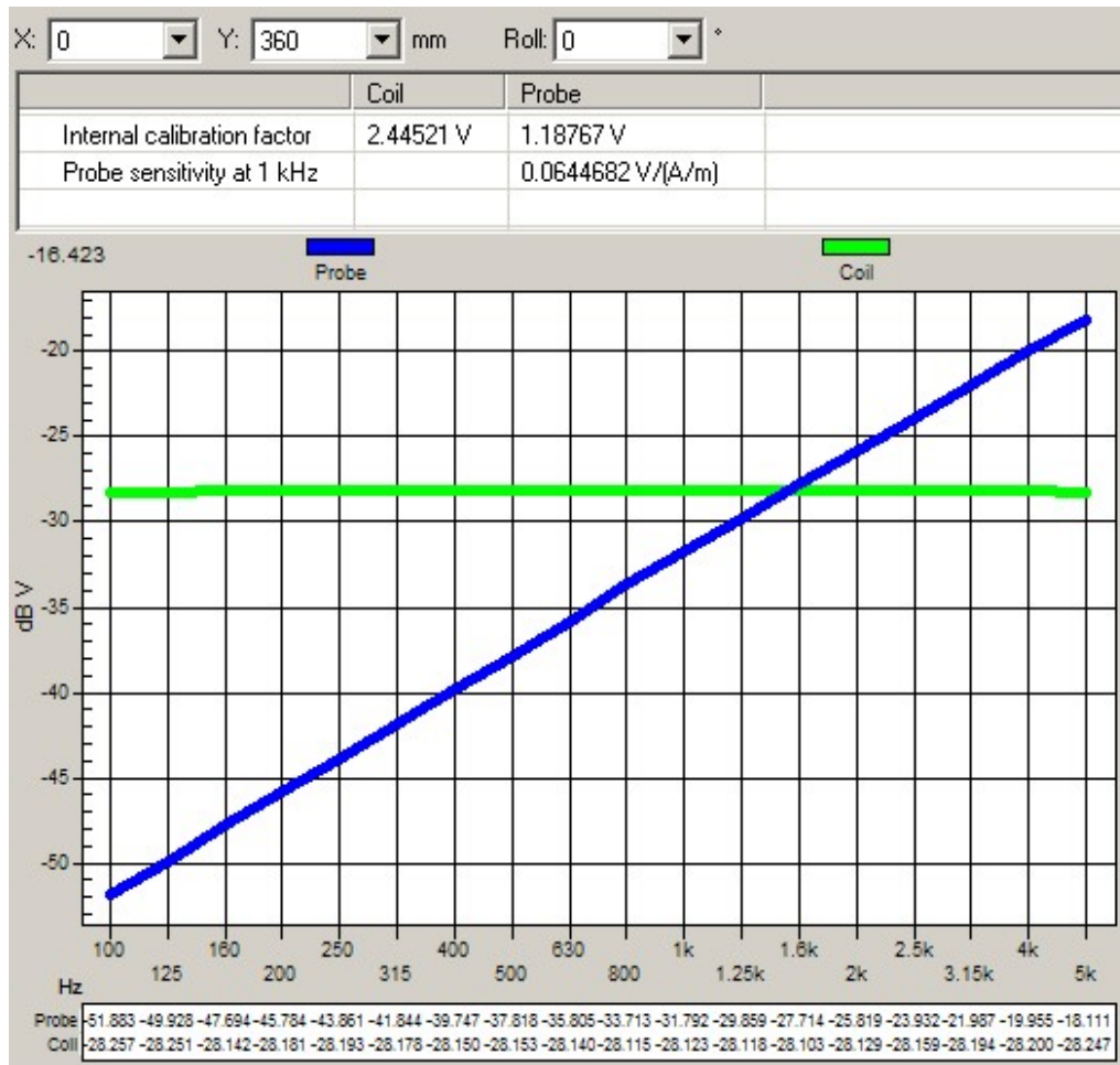
Graph 1: Frequency Response measured in AMCC
