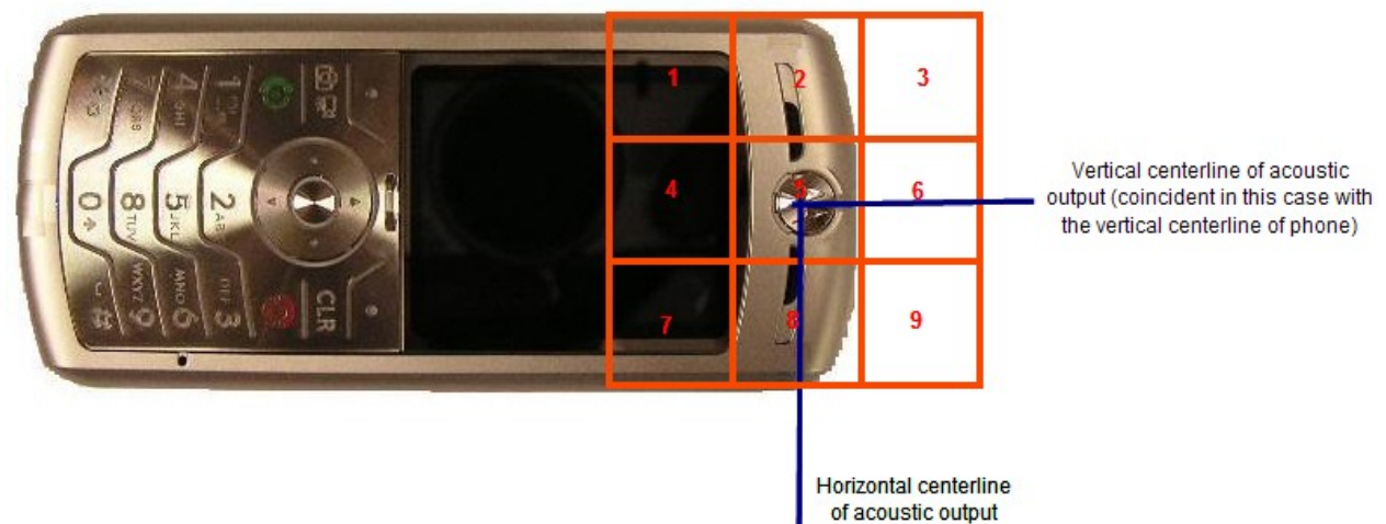
Figure A4-3. Phone Open – 5cm x 5cm grid for Near Field Measurements
