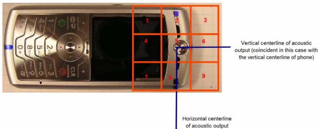
Figure A6-1. Phone Open - Orientation of Wireless Device and Measurement Plane
