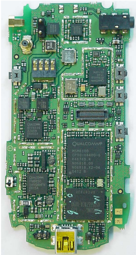
Figure 1: Board with Shields Removed
