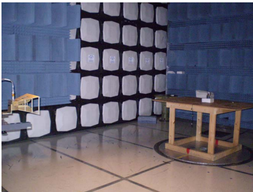
Figure 3.Part 22/24 Radiated Emissions Measurement Setup
