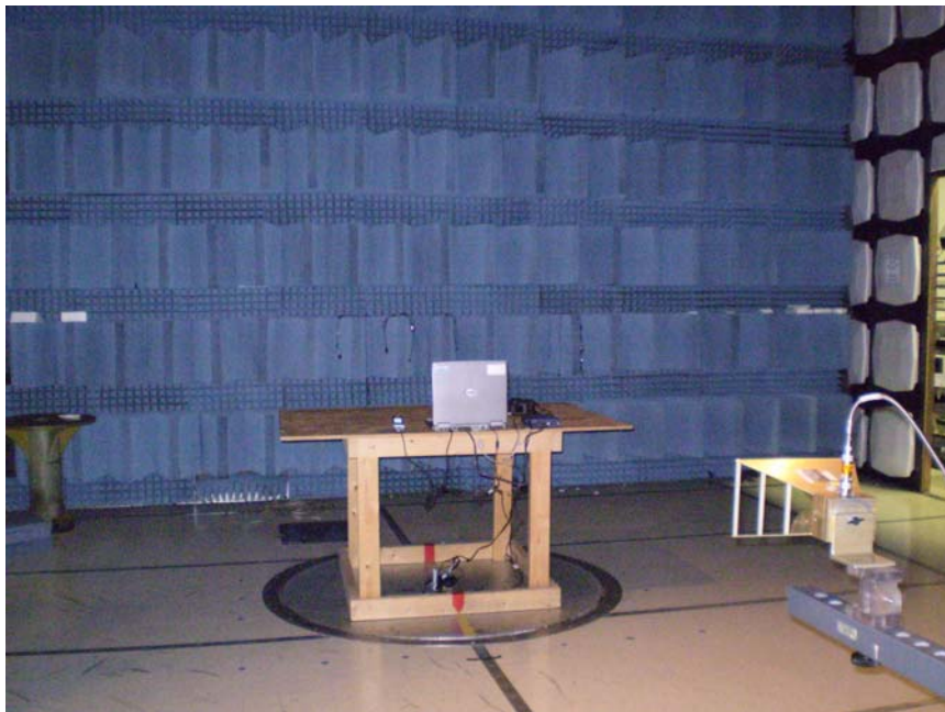
Figure 2. Part 15 Radiated Emissions Measurement Setup
