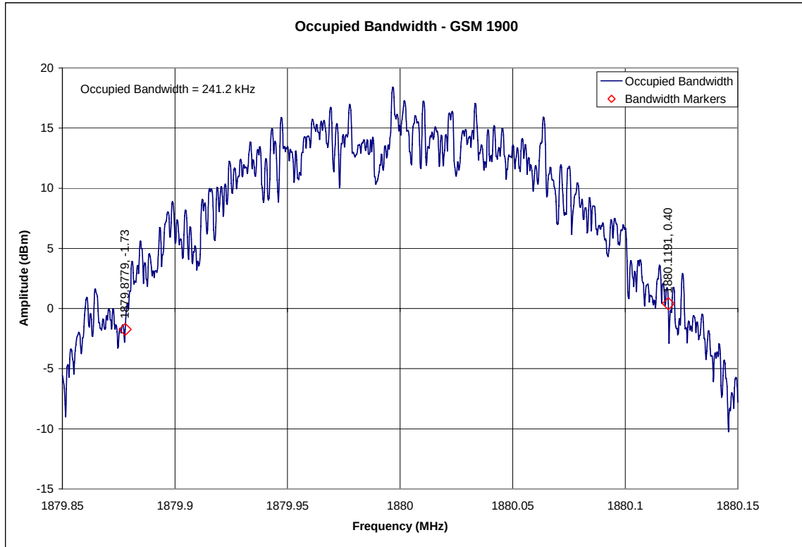
GSM 1900 Edge Occupied Bandwidth
