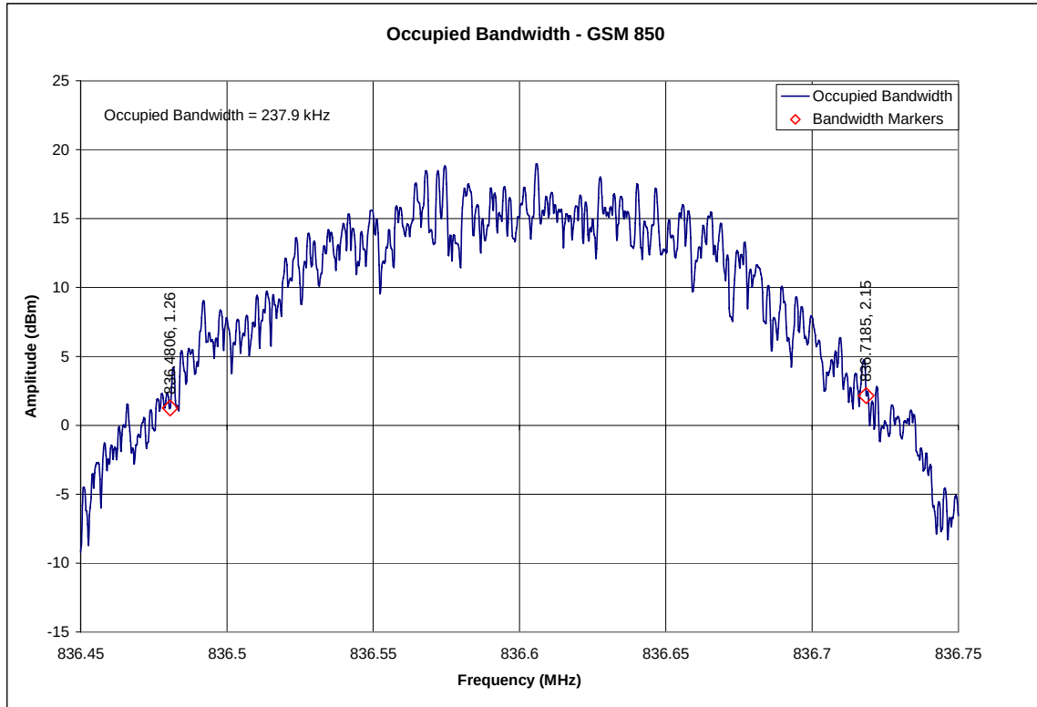
GSM 850 Edge Occupied Bandwidth
