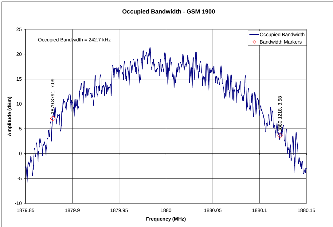
GSM 1900 Occupied Bandwidth
