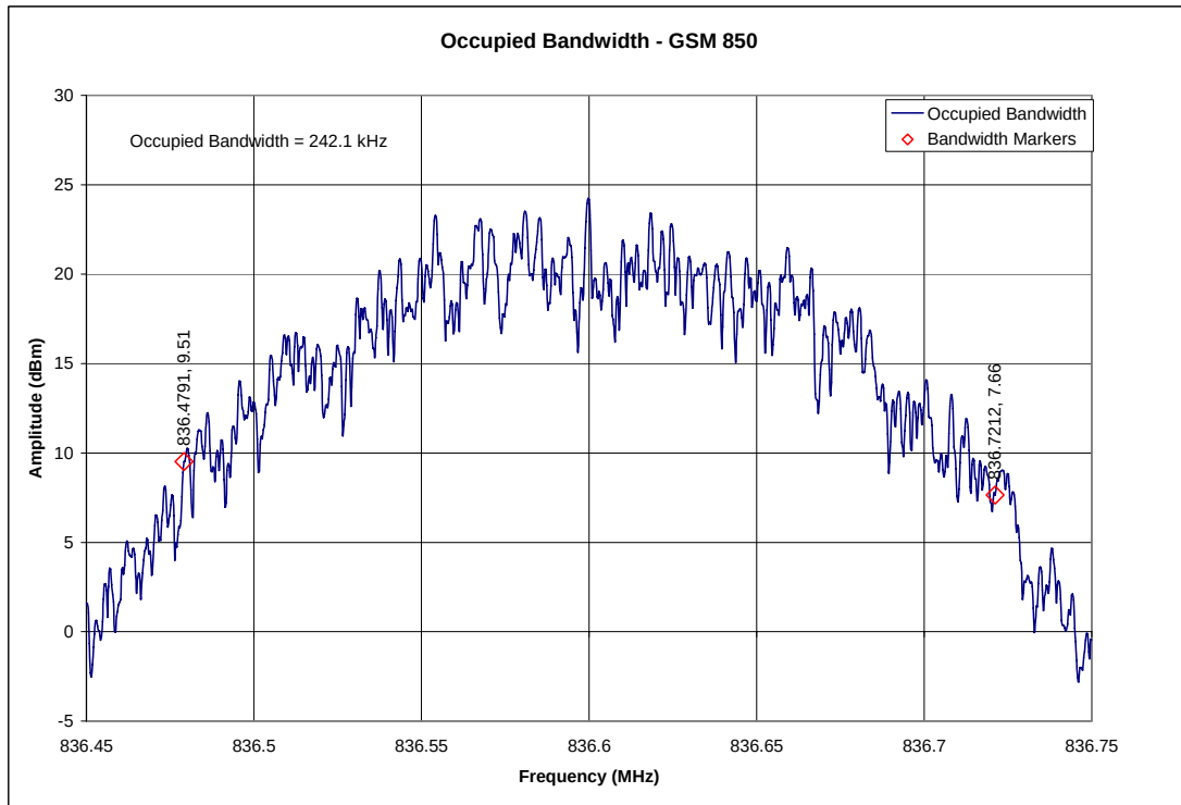
GSM 850 Occupied Bandwidth
