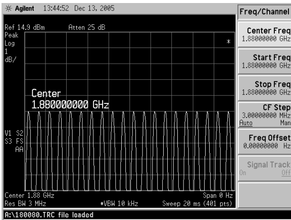
80% AM 1880 MHz
