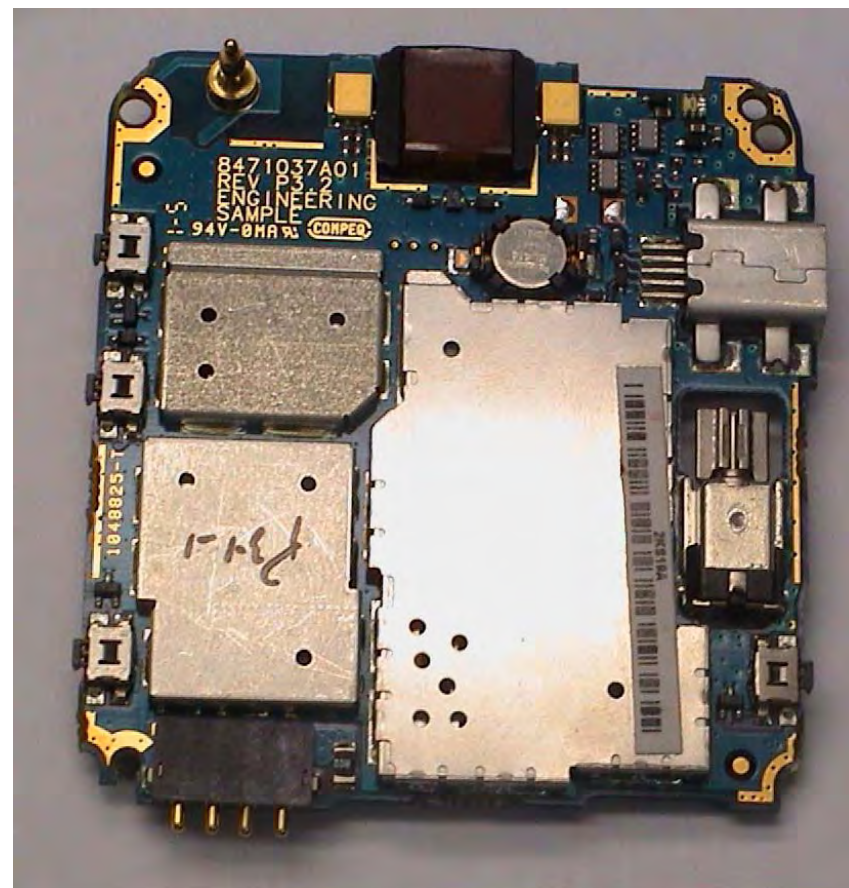
Main PCBA (Rear View)
