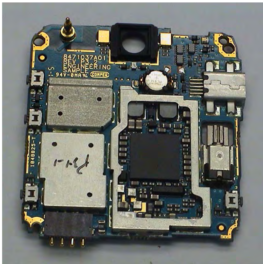
Rear View With Shields Removed
