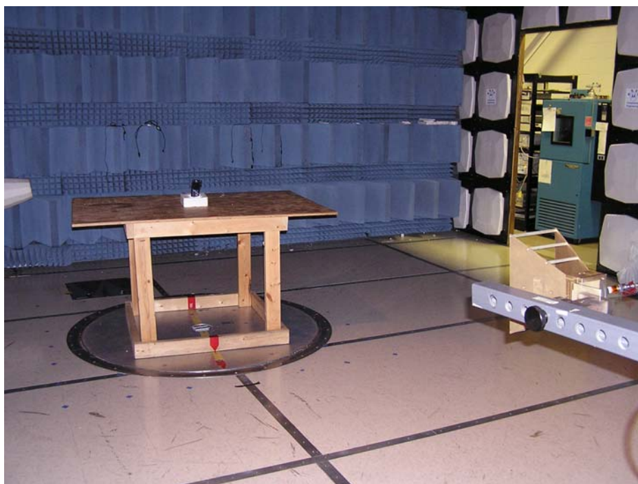
Figure 3. Part 22/24 Radiated Emissions Measurement Setup
