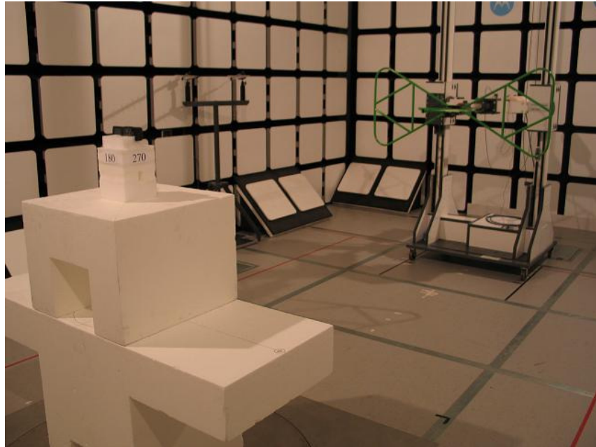
21467-1, IHDT56JA1 setup in semi-anechoic chamber – front view
