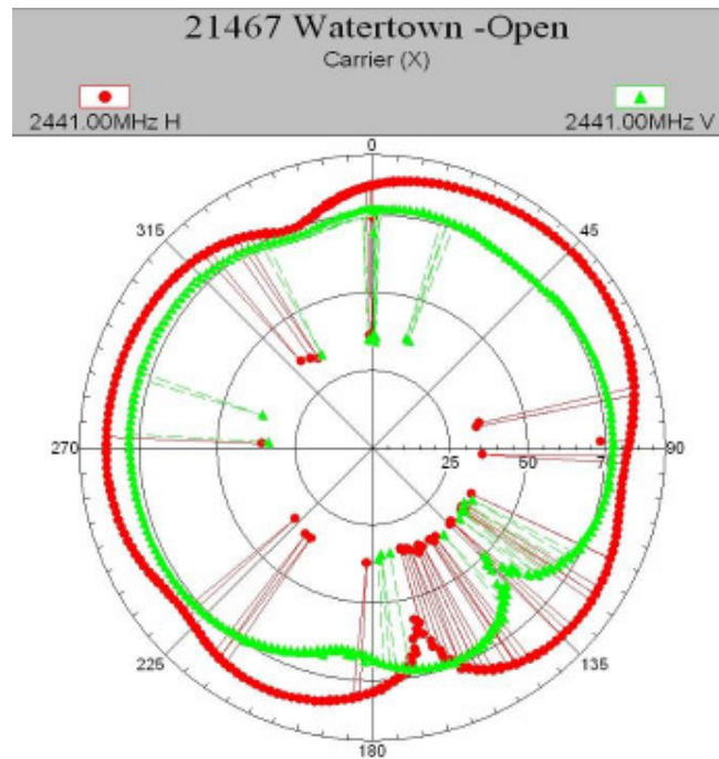
21467-1, IHDT56JA1 maximum radiation pattern position X - Open
