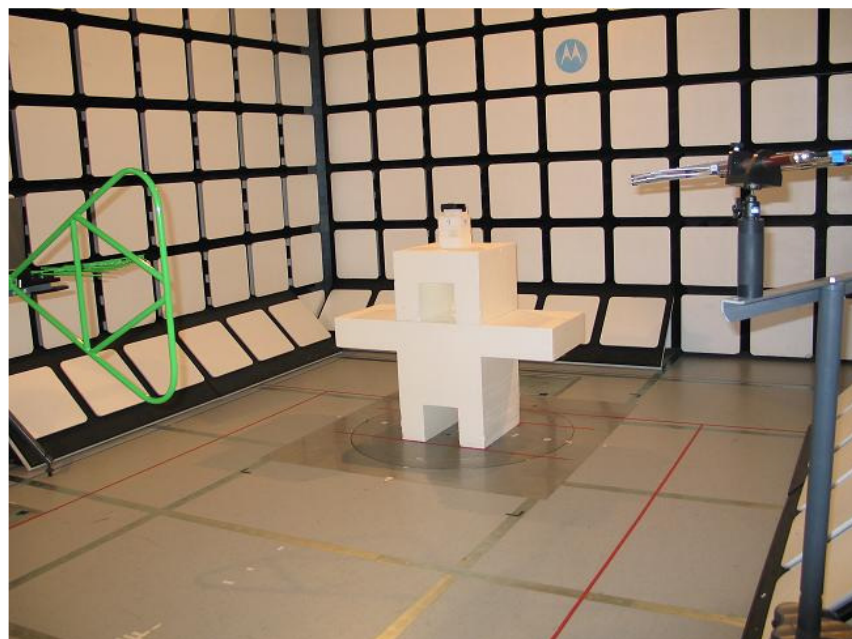
21467-1, IHDT56JA1 setup in semi-anechoic chamber – back view
