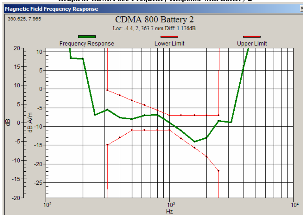
Graph 3: CDMA 800 Frequency Response with Battery 2
