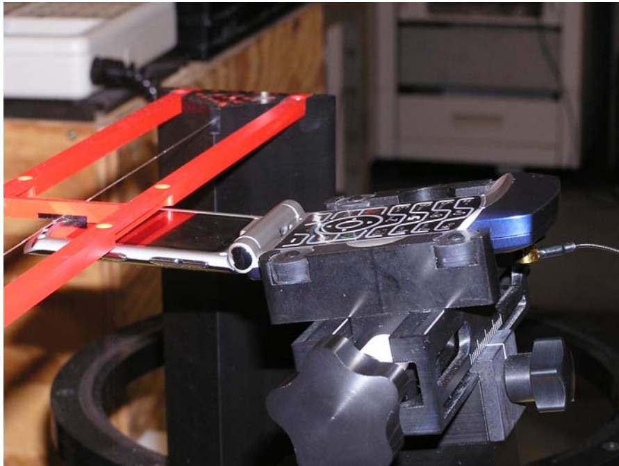
Figure A4-6. Positioning and Measurement for T-coil
