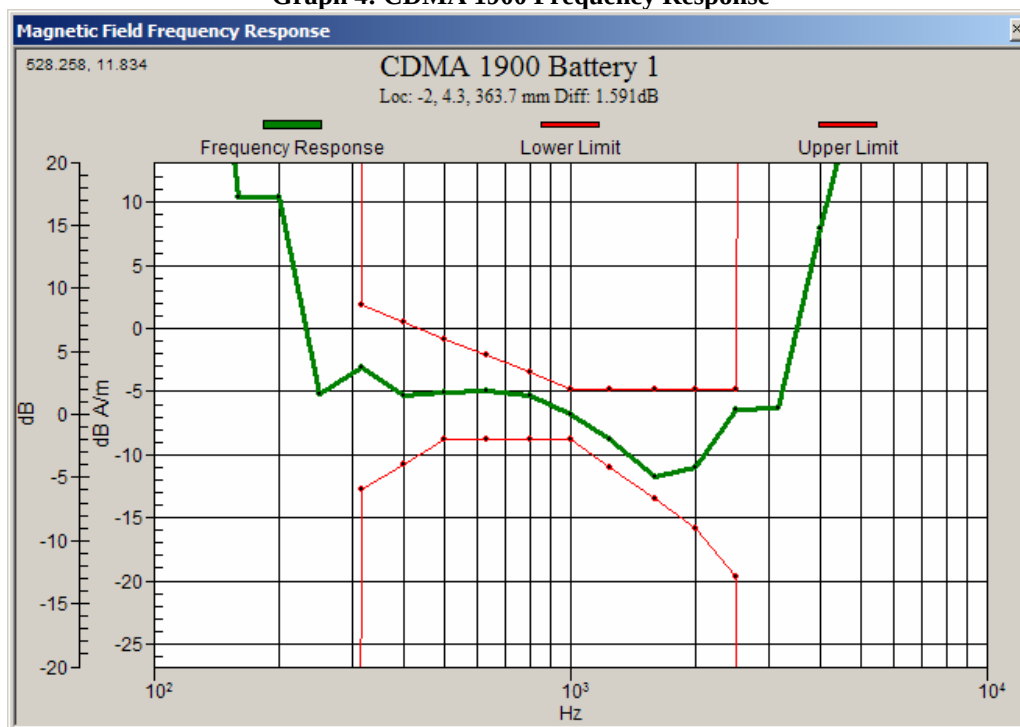
Graph 4: CDMA 1900 Frequency Response
