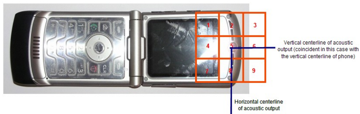
Figure A4-3. Phone Open - Orientation and Measurement Plane for RF Emissions Testing
