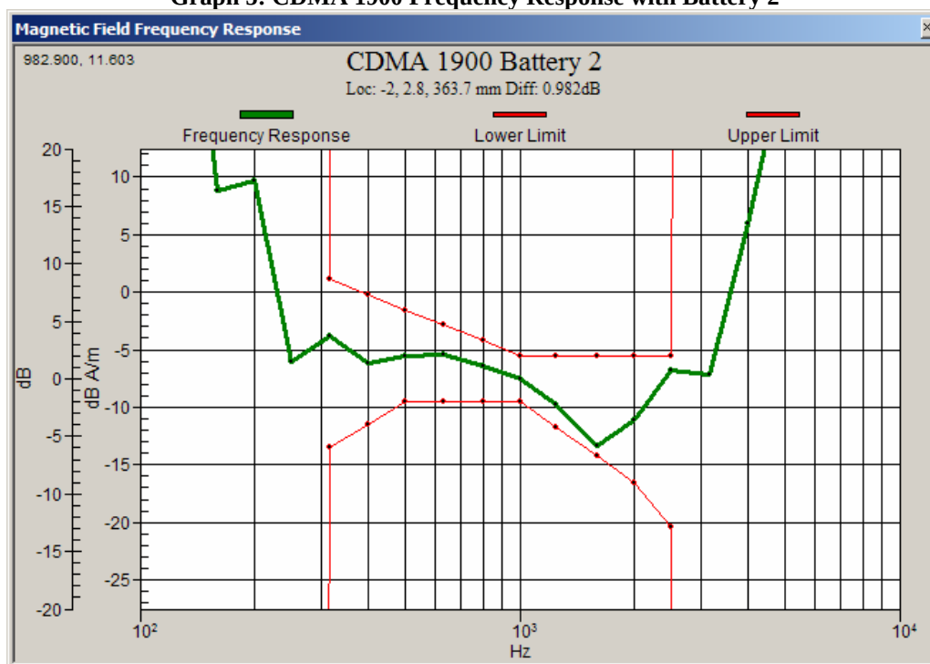
Graph 5: CDMA 1900 Frequency Response with Battery 2
