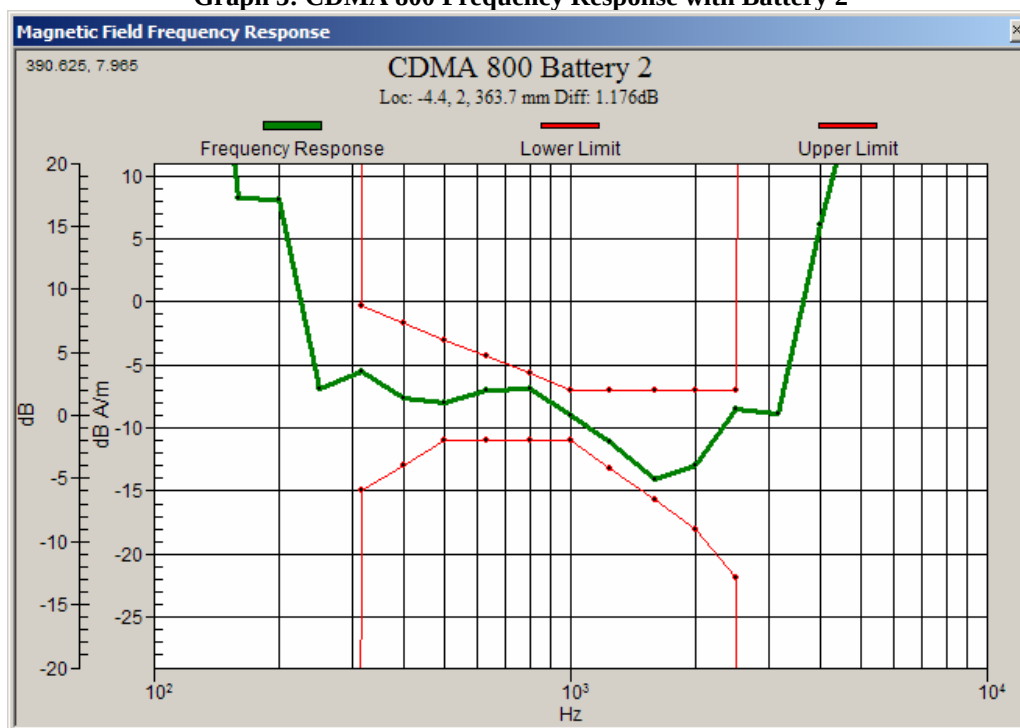
Graph 3: CDMA 800 Frequency Response with Battery 2
