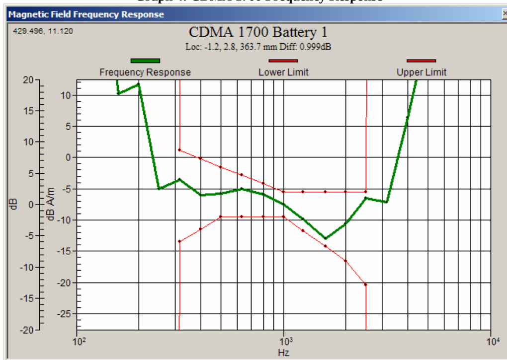
Graph 4: CDMA 1700 Frequency Response
