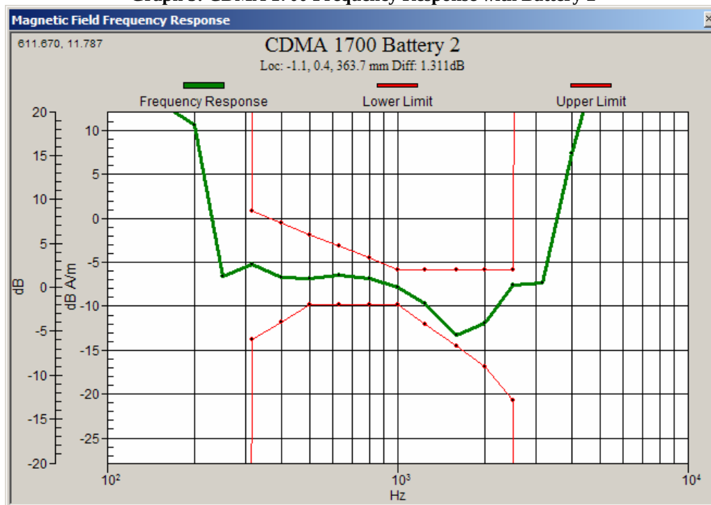
Graph 5: CDMA 1700 Frequency Response with Battery 2
