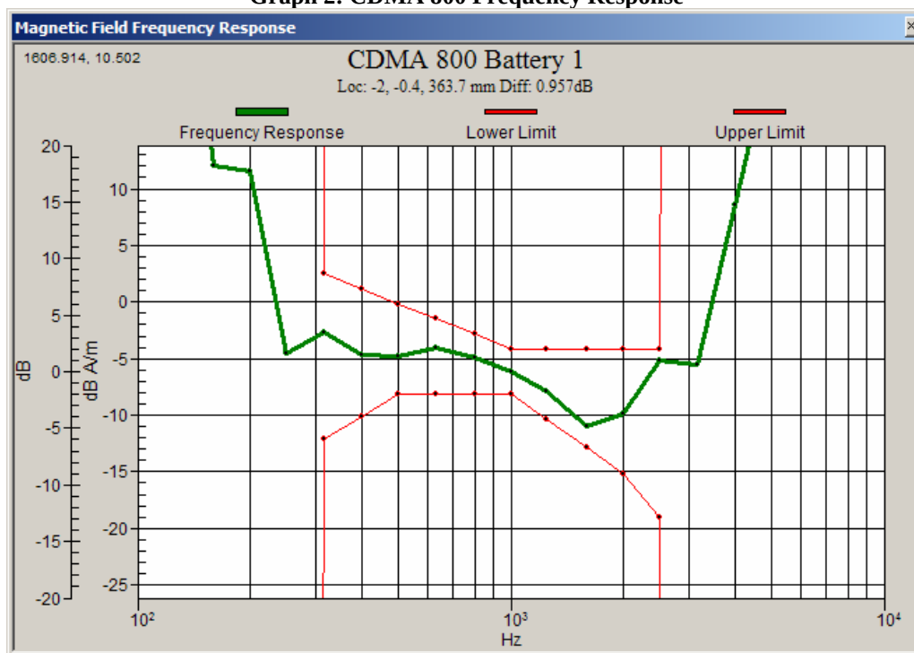
Graph 2: CDMA 800 Frequency Response
