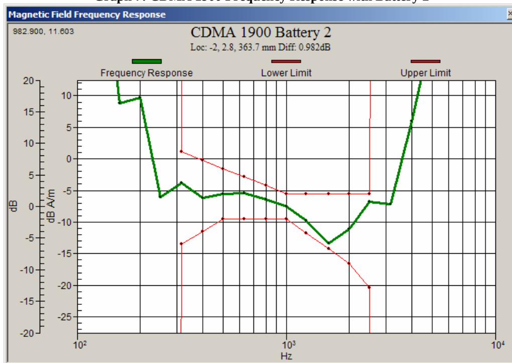
Graph 7: CDMA 1900 Frequency Response with Battery 2
