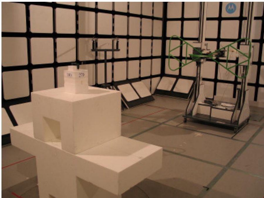
21653-1, IHDT56JT1 setup in semi-anechoic chamber – front view
