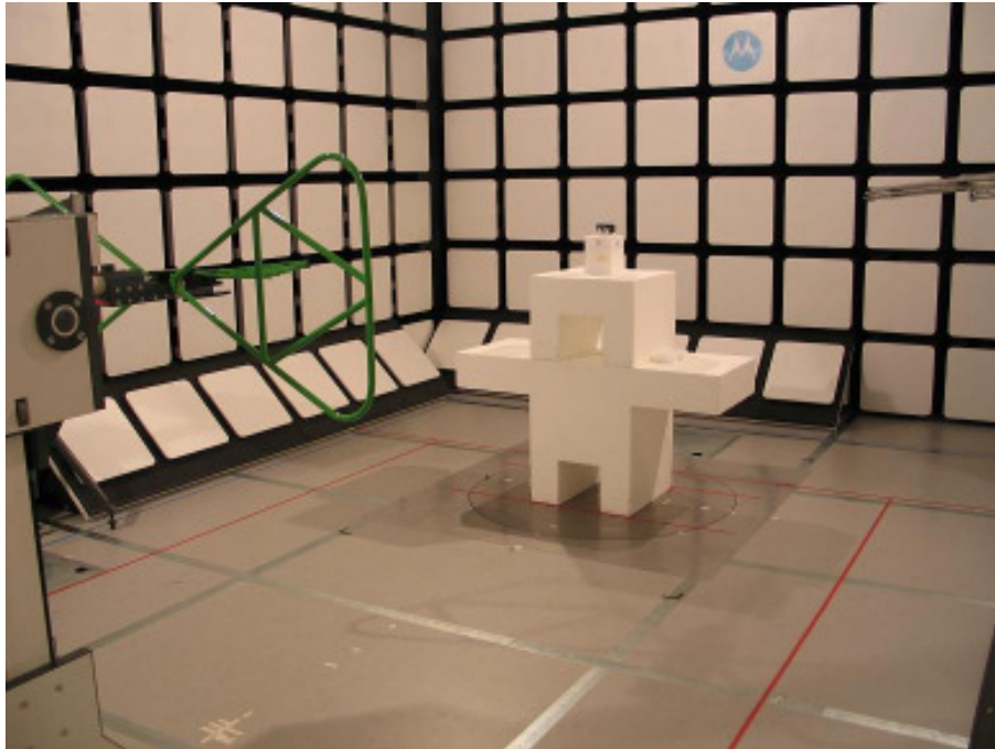
21653-1, IHDT56JT1 setup in semi-anechoic chamber – back view
