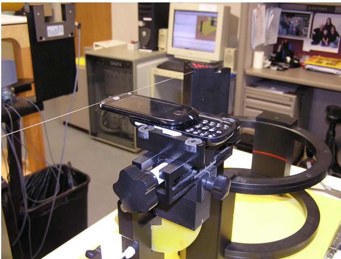
Figure 5. Measurement for RF Emissions
