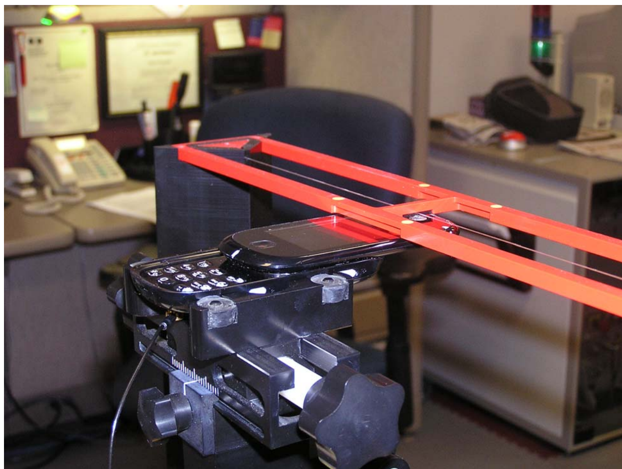
Figure 8. Positioning and Measurement for T-coil
