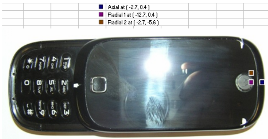
Figure 7. Location of Measured Points for T-coil measurements
