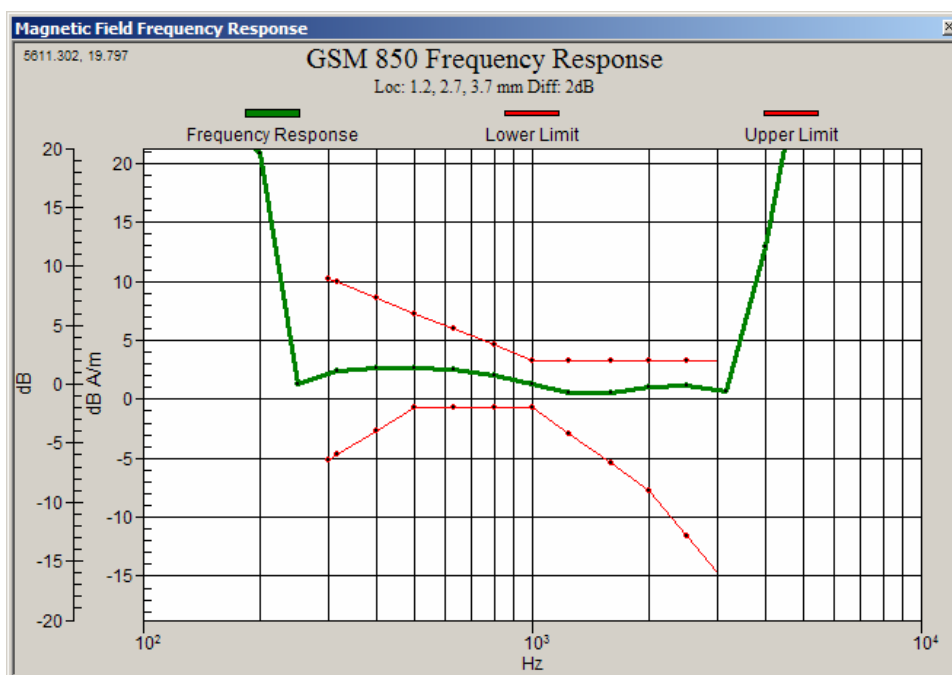
Graph 2: GSM 850 Frequency Response
