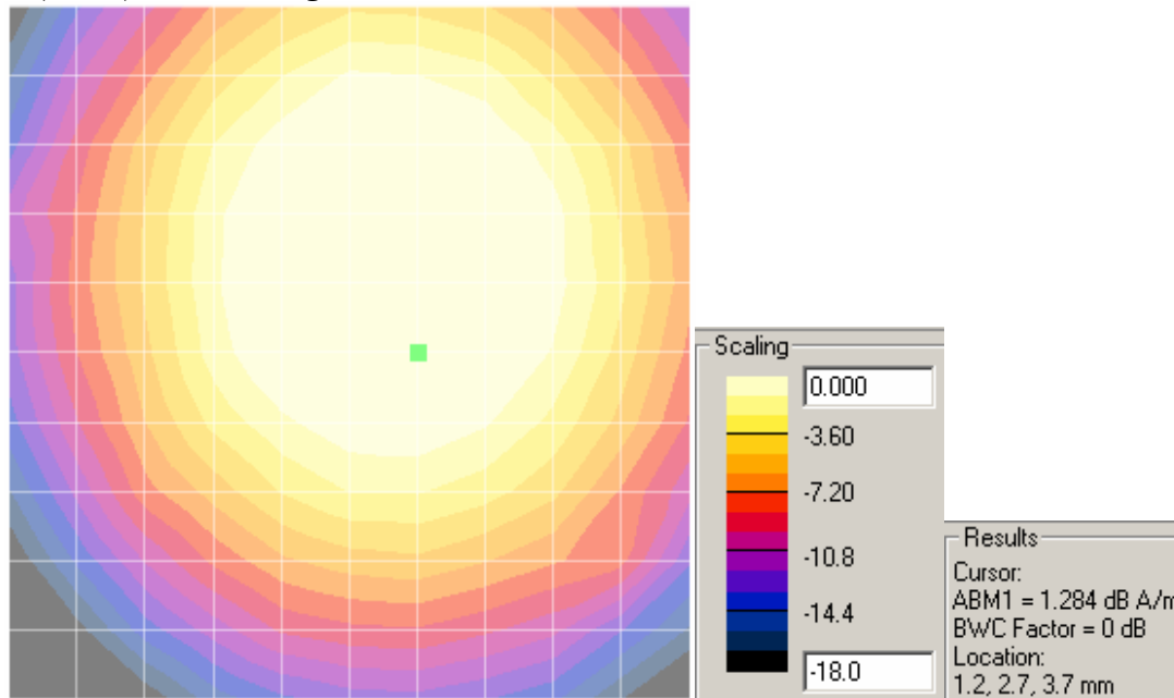
Z (Axial) – ABM1 Signal
