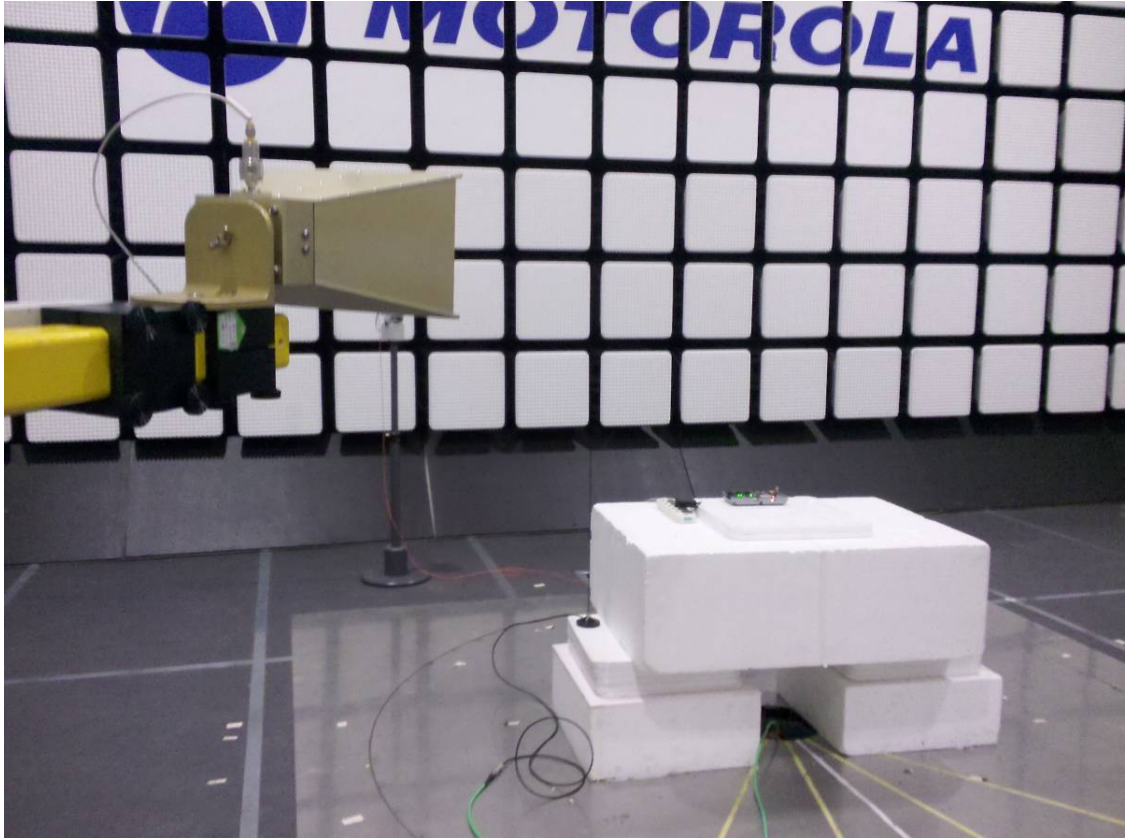
Radiated Emissions
