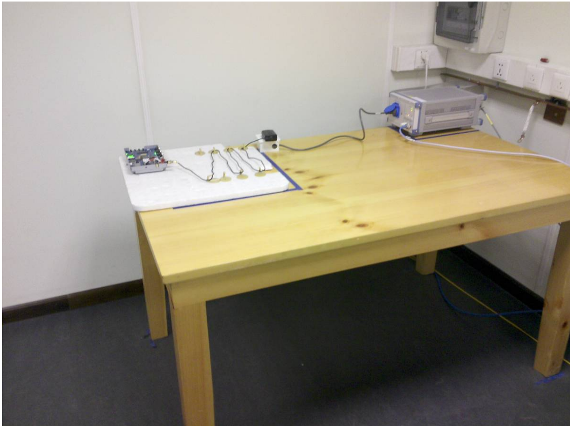
AC Lines Conducted Emissions
