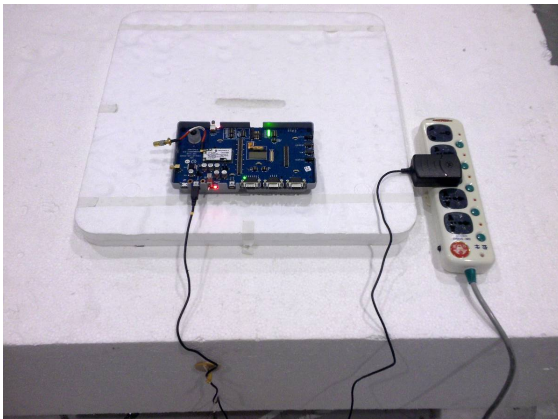
H24 with Evaluation Board 8488899V01_P3
