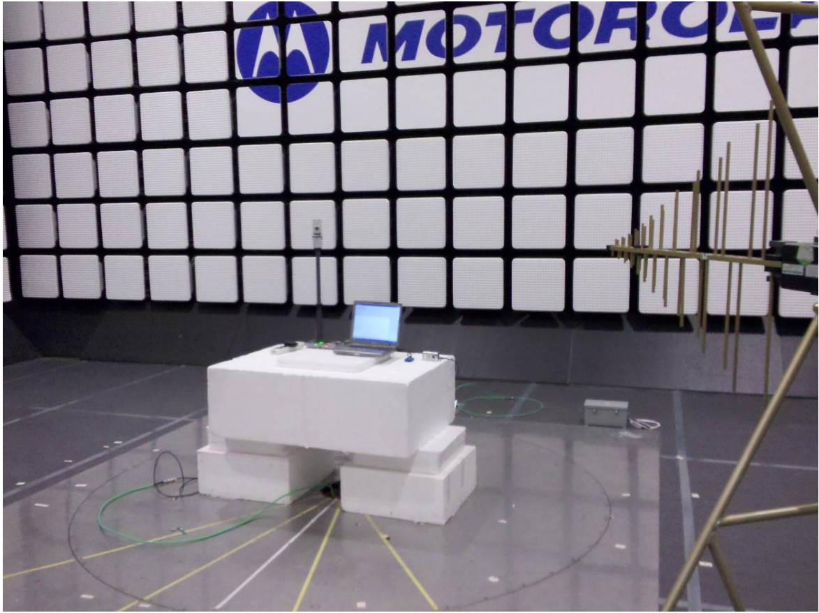
Radiated Emissions – Computer Peripheral
