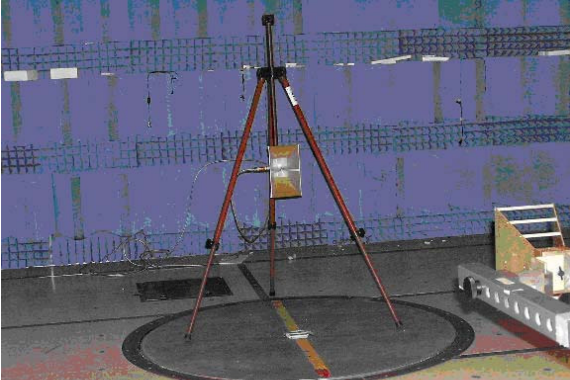
EMC Report #23634Antenna - Substitution
