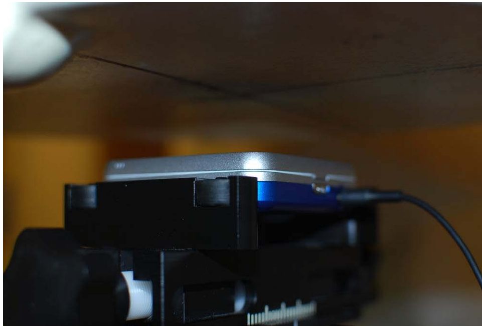
Figure 20-6 SAR Test Setup Photo 6
