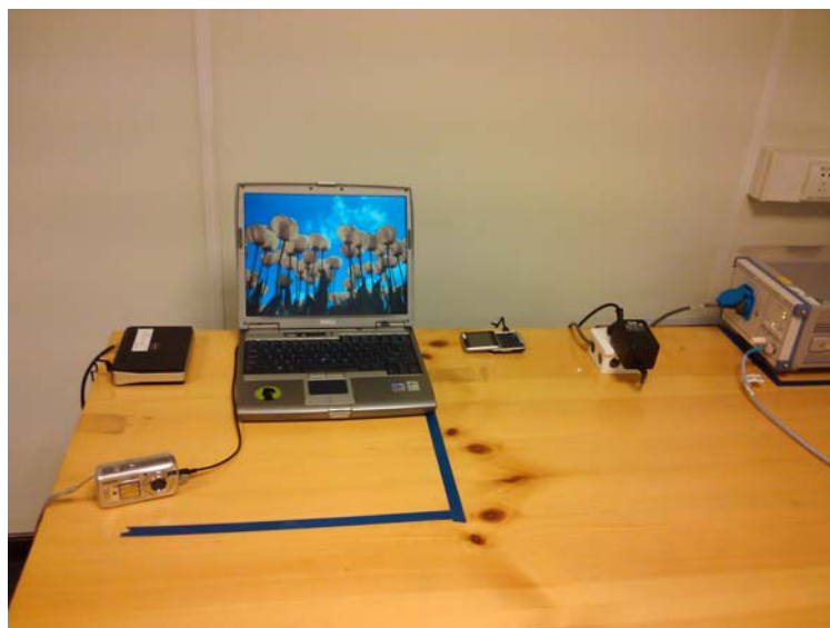
AC Line Conducted Emissions – Computer Peripheral
