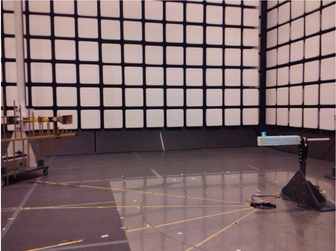
Radiated Emissions
