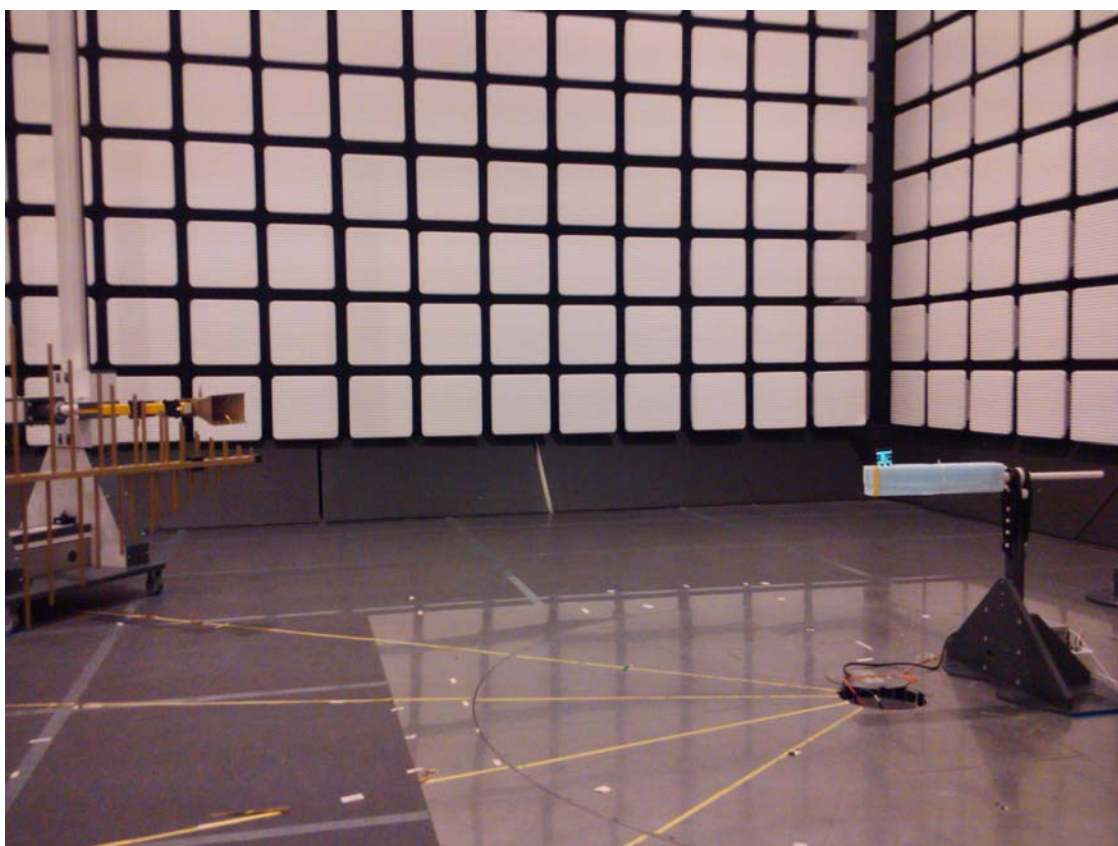
Radiated Emissions
