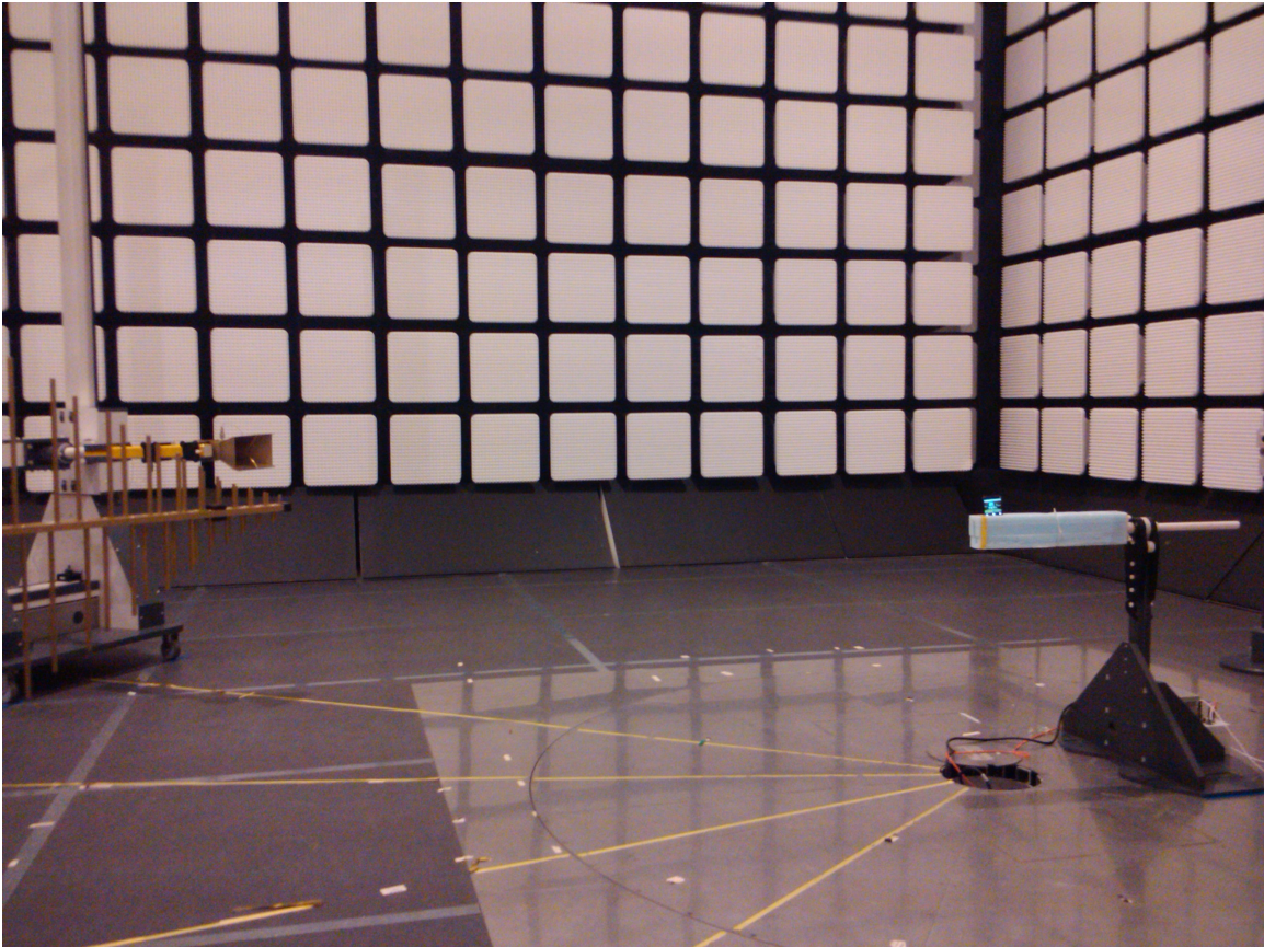
Radiated Emissions – BT & WLAN
