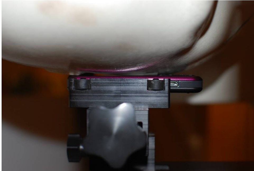
Figure 20-1 SAR Test Setup Photo 1
