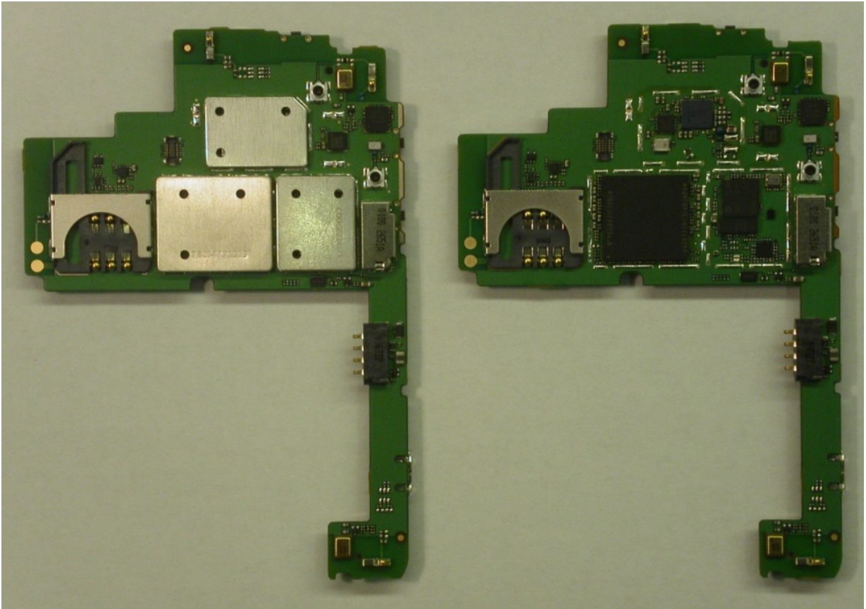
Main Board Bottom With Shields
