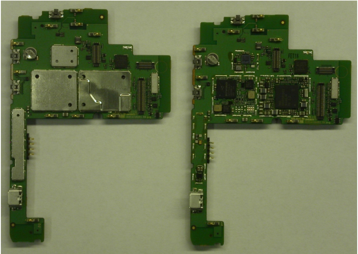
Main Board Top With Shields
