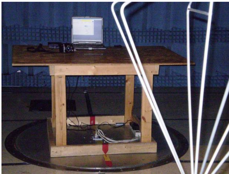
Radiated Emissions - Part 15 PC Peripheral
