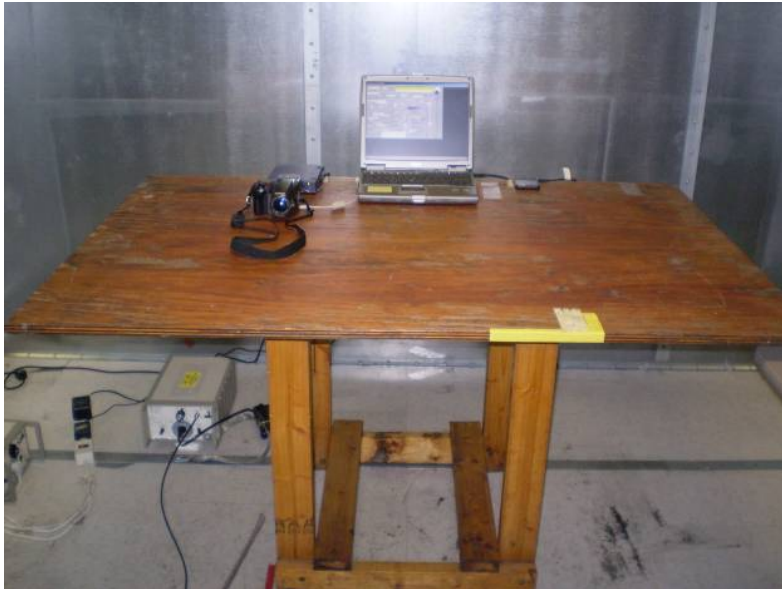
AC Line Conducted Emissions - Part 15 PC Peripheral
