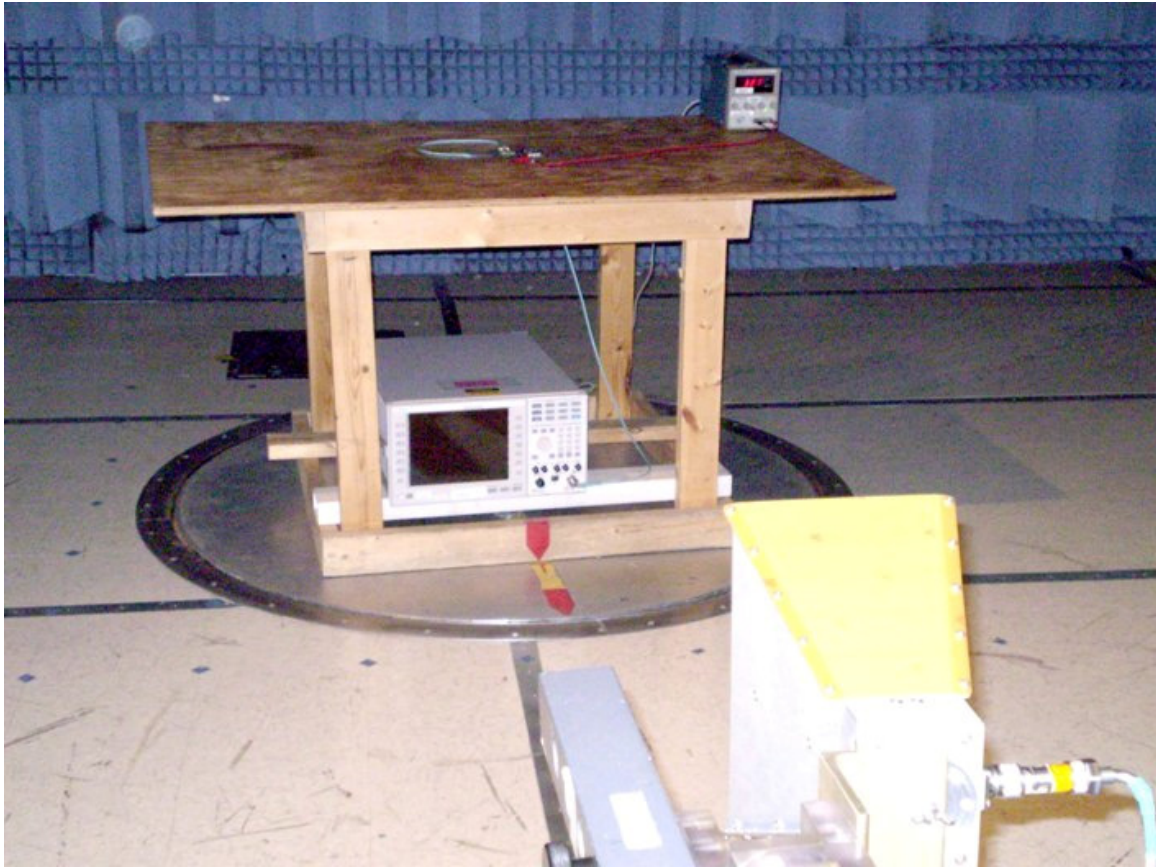
EMC Report #23574 Tx Radiated front view
