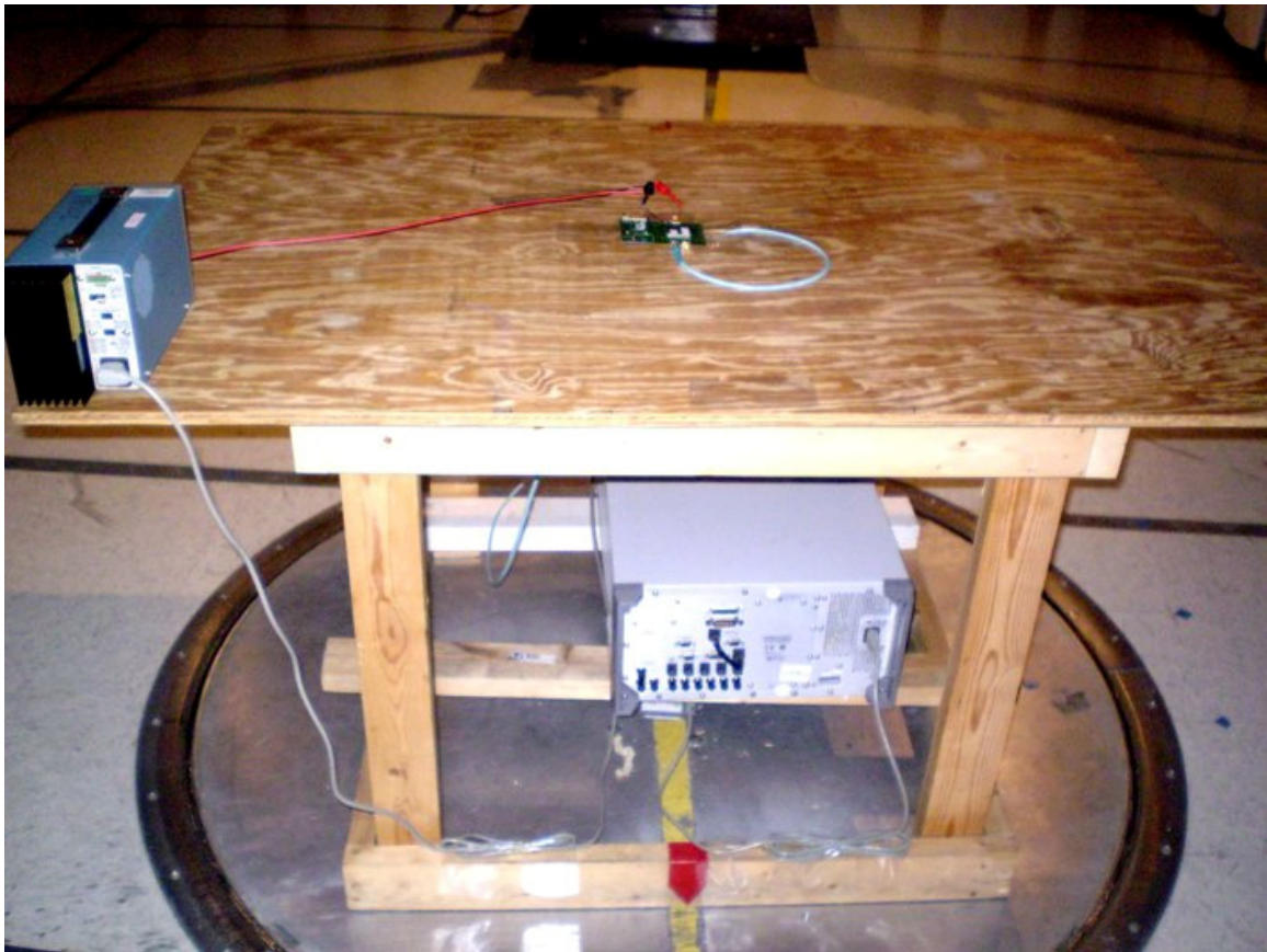
EMC Report #23574 Tx Radiated rear view
