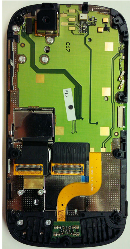
Front Subassembly with PCB removed
