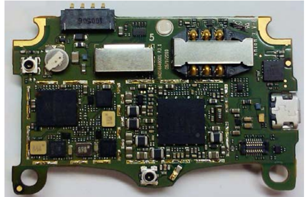
Main Board Bottom Without Shields
