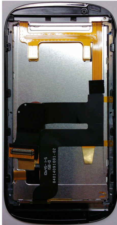
Slide Assembly with Display and Flexes (Slide-Plate removed)
