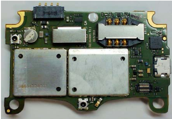
Main Board Bottom With Shields
