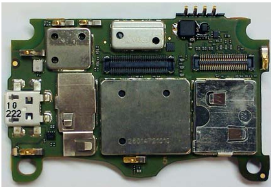
Main Board Top With Shields
