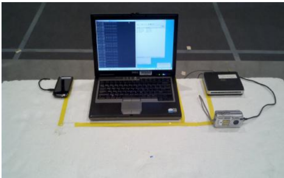
Radiated Emissions – Computer Peripheral
