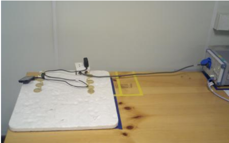
AC Line Conducted Emissions
